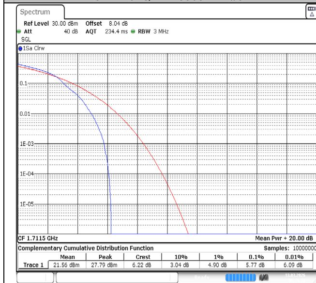
Band4-3MHz-64QAM-19965-1RB#0-PASS
