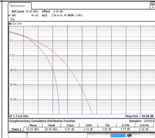
Band4-3MHz-16QAM-19965-15RB#0-PASS
