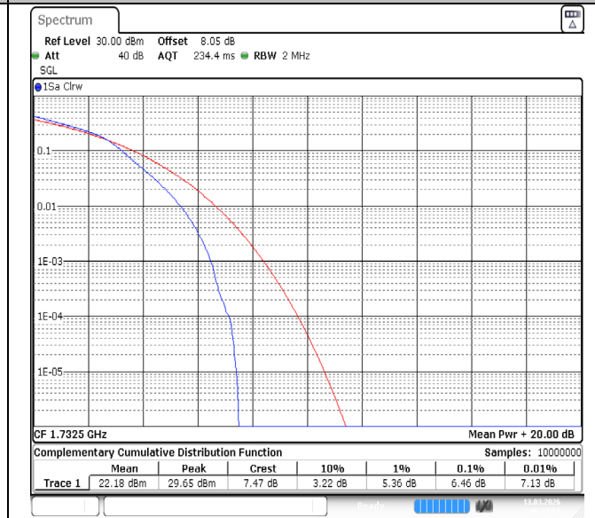
Band4-1.4MHz-16QAM-20175-6RB#0-PASS
