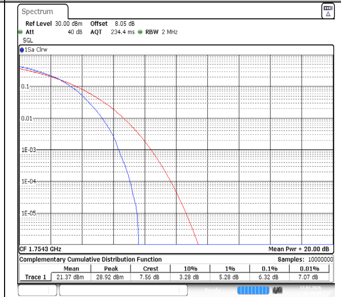
Band4-1.4MHz-64QAM-20393-6RB#0-PASS
