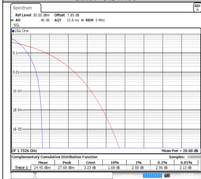
Band4-1312-PASS
