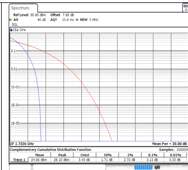
Band4-1413-PASS
