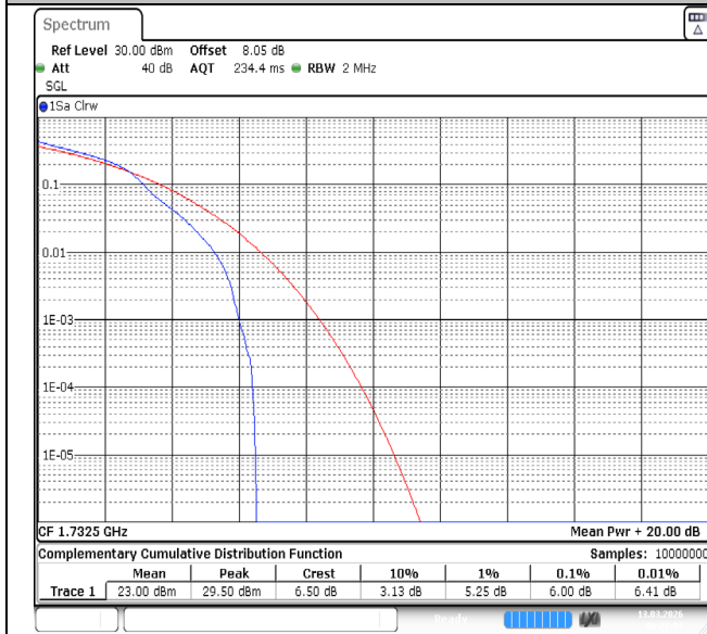
Band4-1.4MHz-64QAM-20175-1RB#0-PASS
