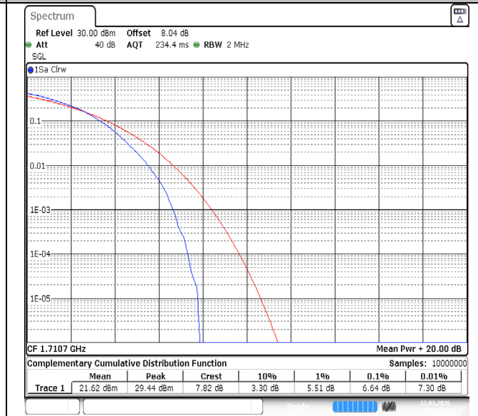
Band4-1.4MHz-64QAM-19957-6RB#0-PASS
