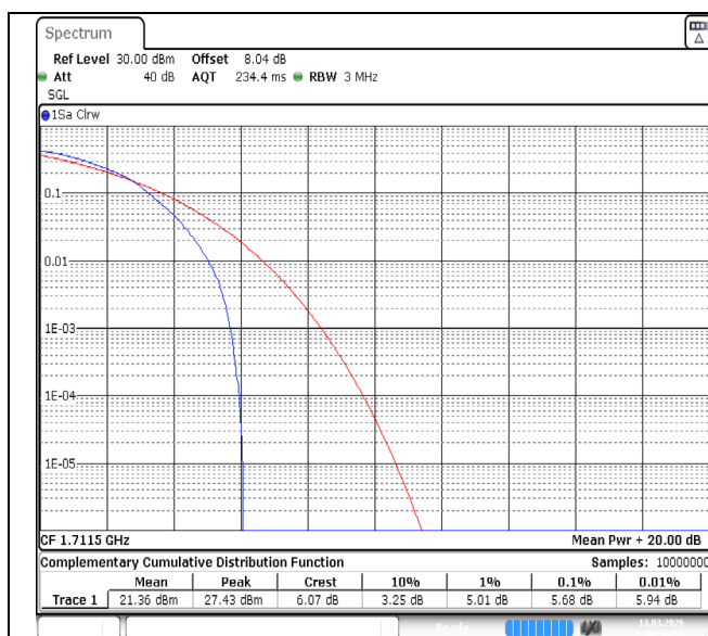
Band4-3MHz-64QAM-19965-1RB#0-PASS
