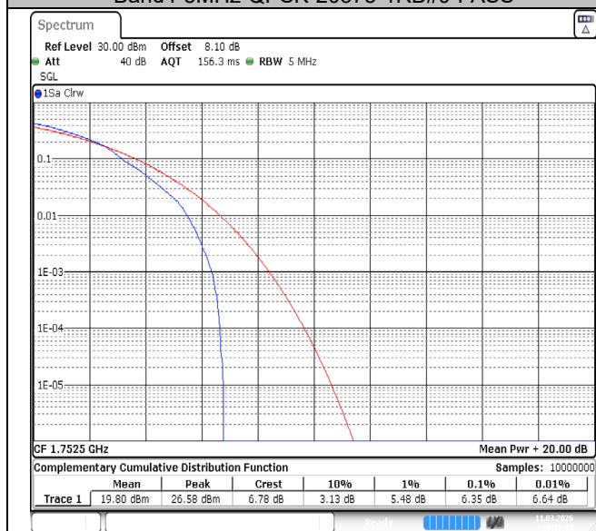
Band4-5MHz-QPSK-20375-1RB#0-PASS
