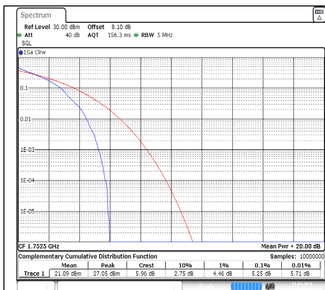
Band4-5MHz-QPSK-20375-1RB#0-PASS
