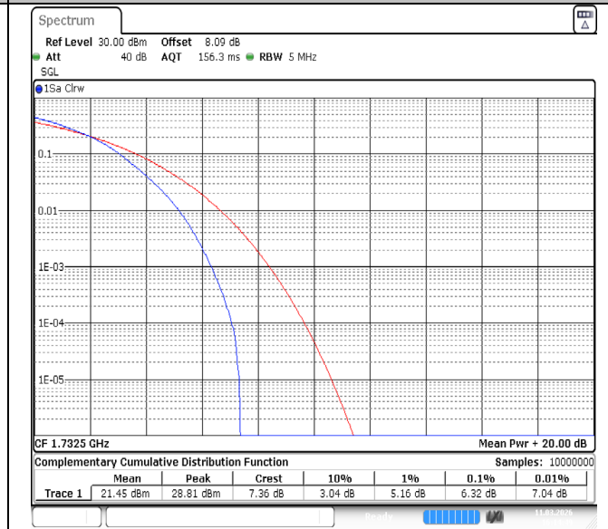
Band4-5MHz-16QAM-20175-25RB#0-PASS
