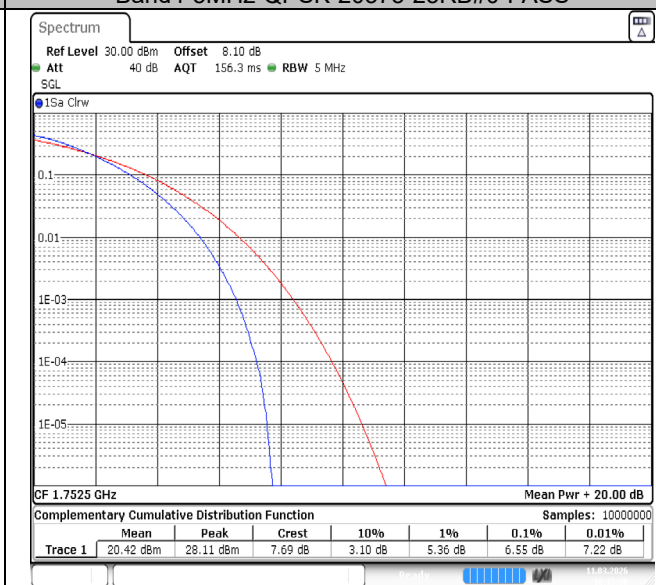
Band4-5MHz-QPSK-20375-25RB#0-PASS
