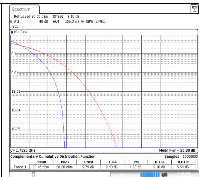
Band4-5MHz-QPSK-20375-25RB#0-PASS
