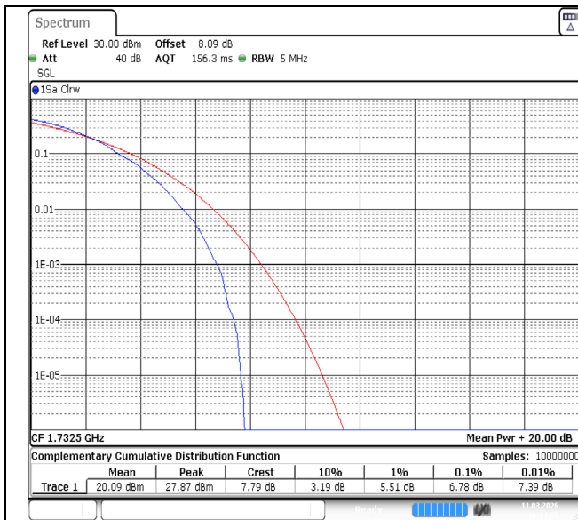
Band4-5MHz-64QAM-20175-1RB#0-PASS
