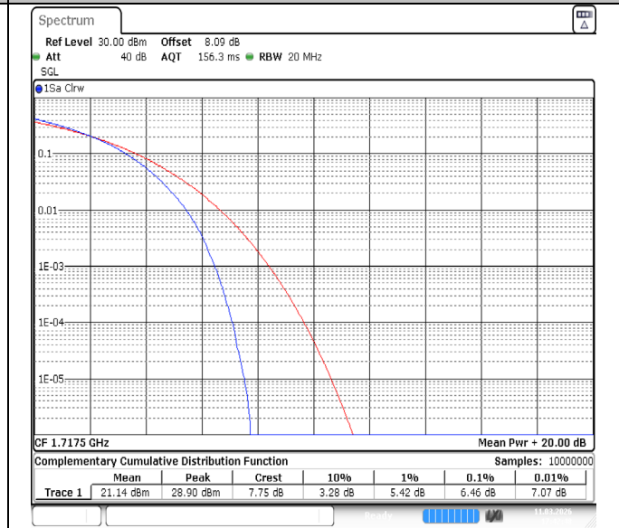
Band4-15MHz-64QAM-20025-75RB#0-PASS
