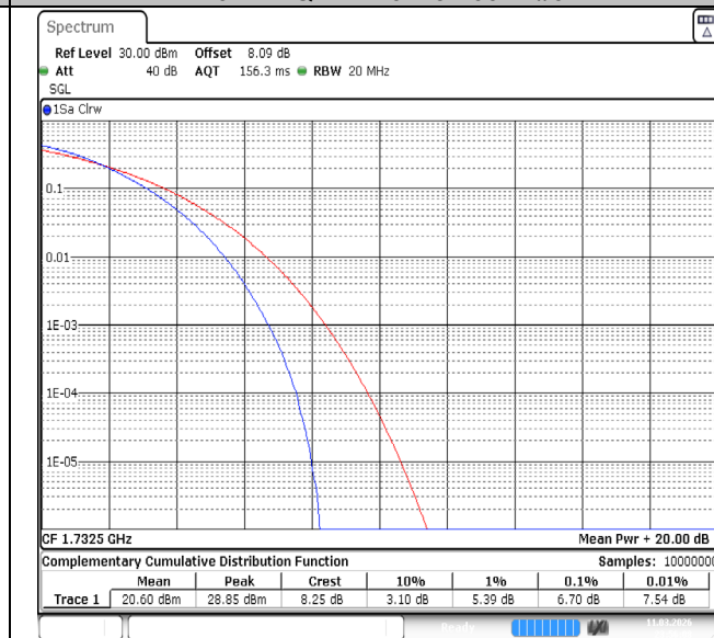
Band4-20MHz-64QAM-20175-100RB#0-PASS
