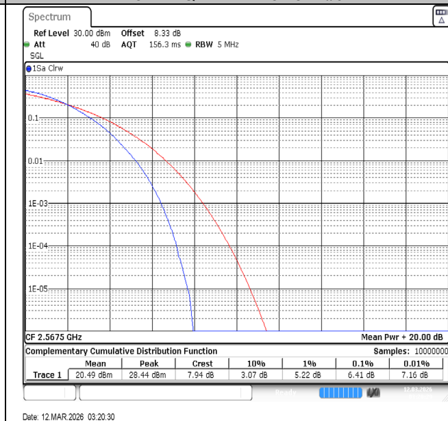
Band7-5MHz-64QAM-21425-25RB#0-PASS
