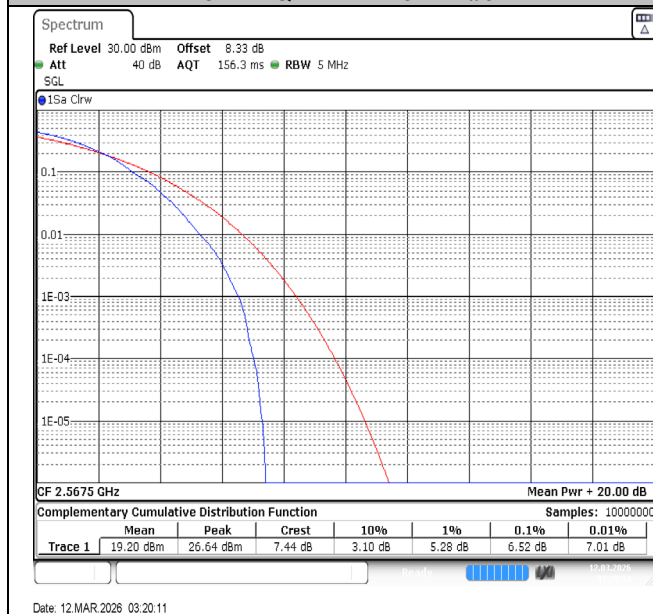
Band7-5MHz-64QAM-21425-1RB#0-PASS
