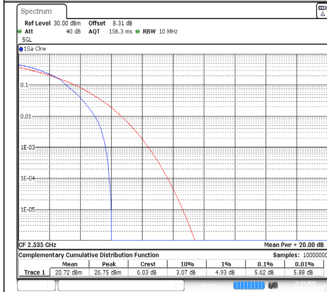
Band7-10MHz-QPSK-21100-1RB#0-PASS
