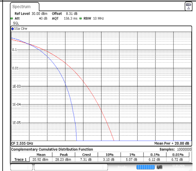
Band7-10MHz-64QAM-21100-50RB#0-PASS
