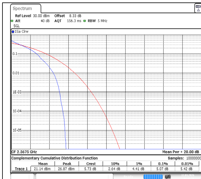
Band7-5MHz-QPSK-21425-1RB#0-PASS
