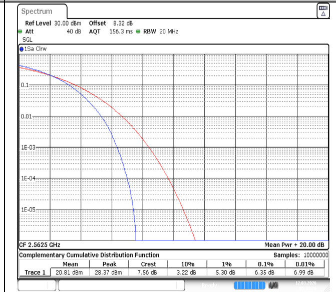
Band7-15MHz-64QAM-21375-75RB#0-PASS
