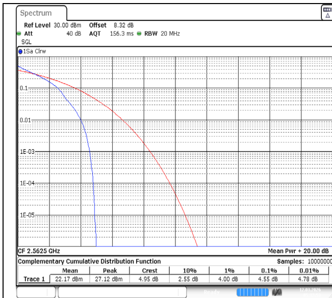
Band7-15MHz-QPSK-21375-1RB#0-PASS
