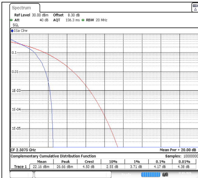
Band7-15MHz-QPSK-20825-1RB#0-PASS
