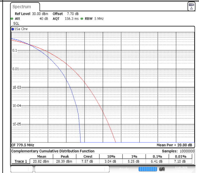
Band13-5MHz-64QAM-23205-25RB#0-PASS
