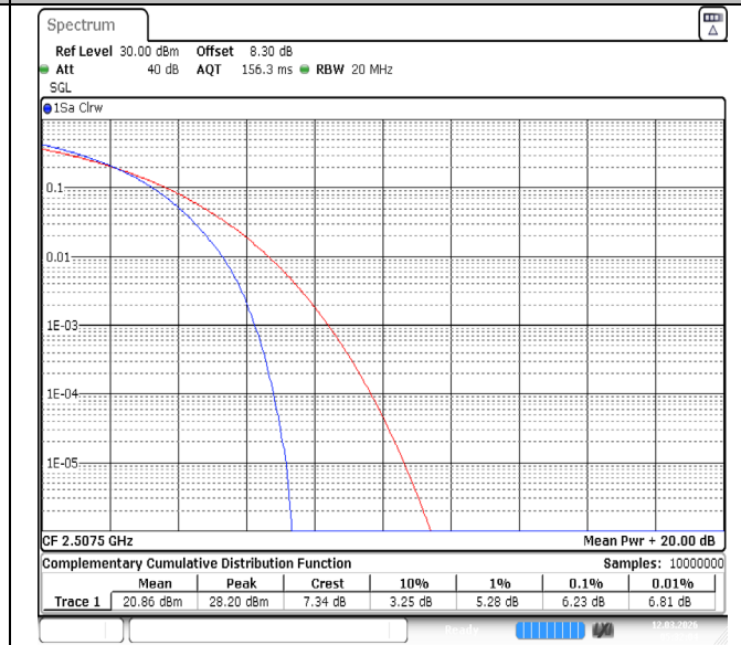
Band7-15MHz-64QAM-20825-75RB#0-PASS
