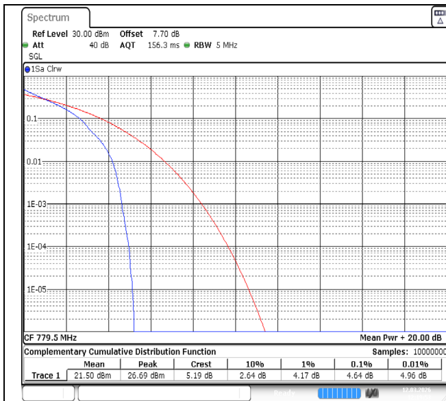
Band13-5MHz-QPSK-23205-1RB#0-PASS
