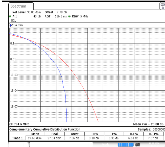
Band13-5MHz-QPSK-23255-1RB#0-PASS
