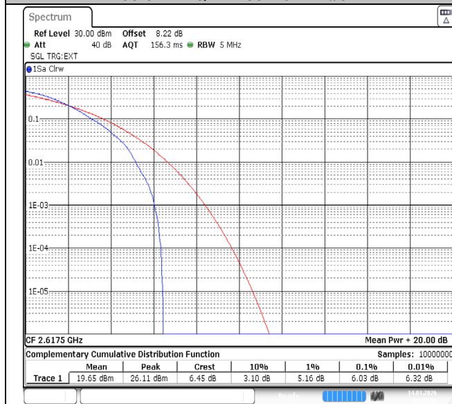
Band38-5MHz-QPSK-38225-1RB#0-PASS
