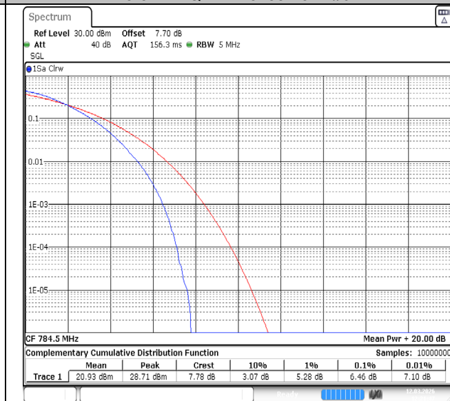
Band13-5MHz-64QAM-23255-25RB#0-PASS
