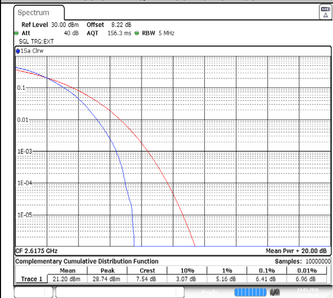
Band38-5MHz-64QAM-38225-25RB#0-PASS
