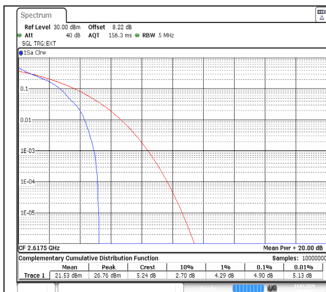
Band38-5MHz-QPSK-38225-1RB#0-PASS
