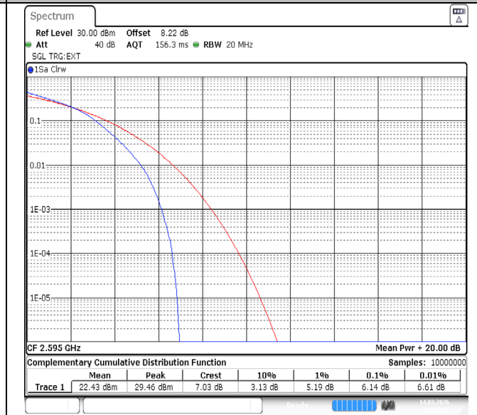
Band38-15MHz-16QAM-38000-75RB#0-PASS
