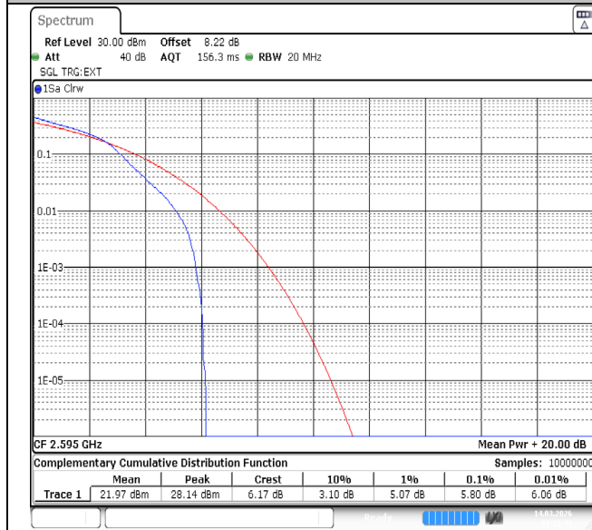
Band38-15MHz-64QAM-38000-1RB#0-PASS
