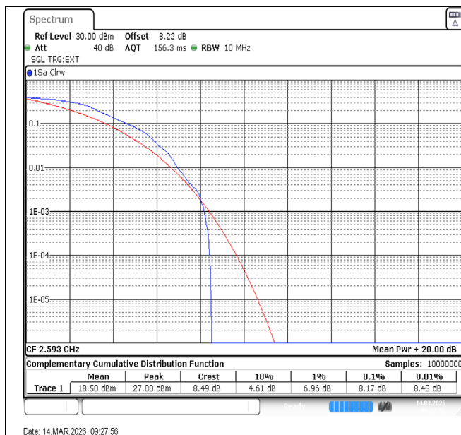
Band41-10MHz-QPSK-40620-1RB#0-PASS
