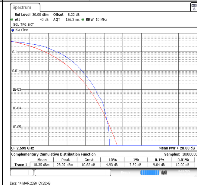
Band41-10MHz-64QAM-40620-50RB#0-PASS
