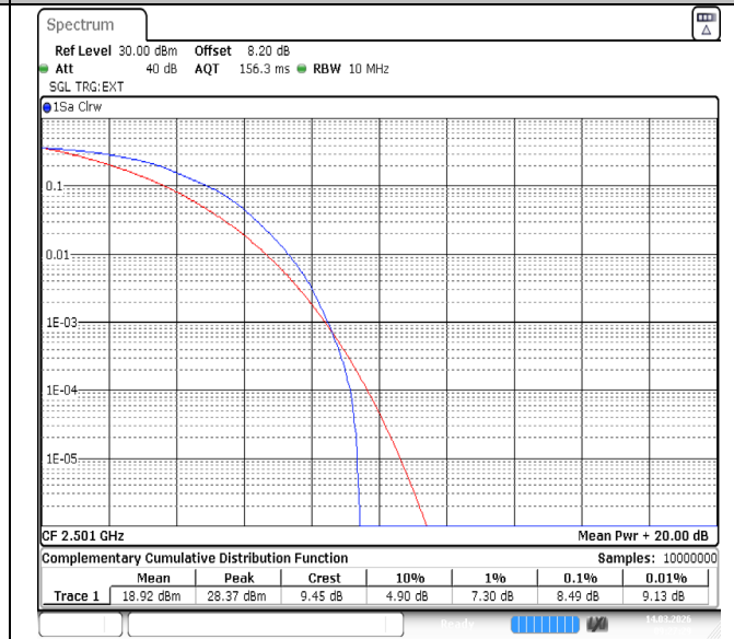
Band41-10MHz-16QAM-39700-50RB#0-PASS
