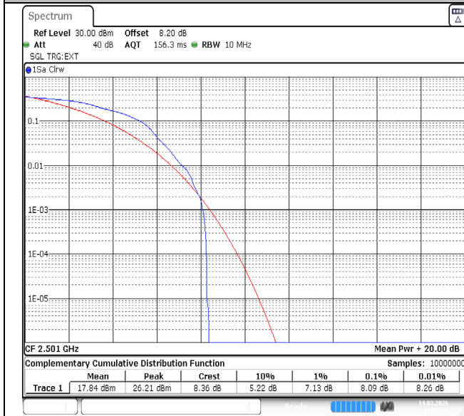
Band41-10MHz-64QAM-39700-1RB#0-PASS
