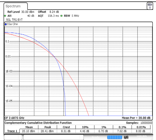
Band41-5MHz-QPSK-41565-25RB#0-PASS
