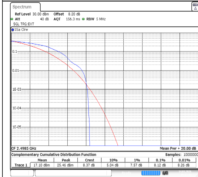
Band41-5MHz-QPSK-39675-1RB#0-PASS
