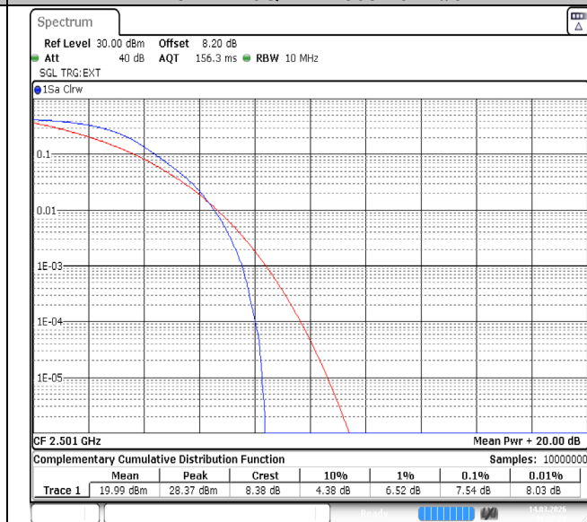
Band41-10MHz-QPSK-39700-50RB#0-PASS
