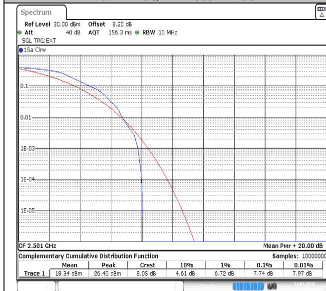
Band41-5MHz-16QAM-41565-1RB#0-PASS
