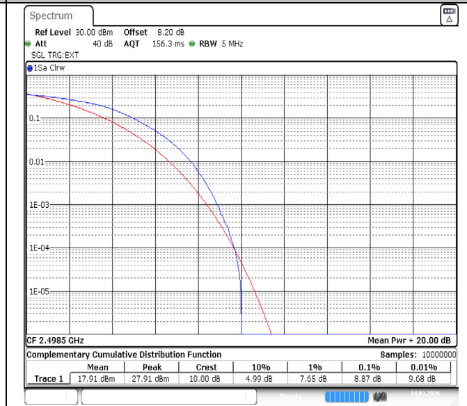
Band41-5MHz-64QAM-39675-25RB#0-PASS
