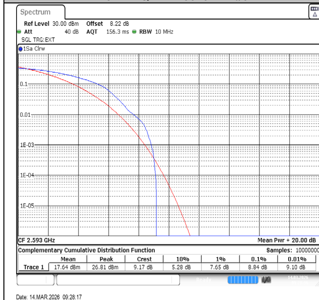
Band41-10MHz-64QAM-40620-1RB#0-PASS
