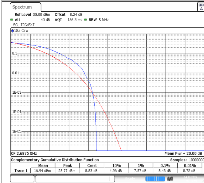
Band41-5MHz-QPSK-41565-1RB#0-PASS
