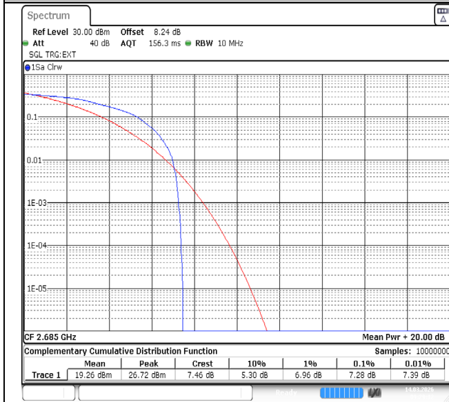
Band41-10MHz-64QAM-41540-1RB#0-PASS
