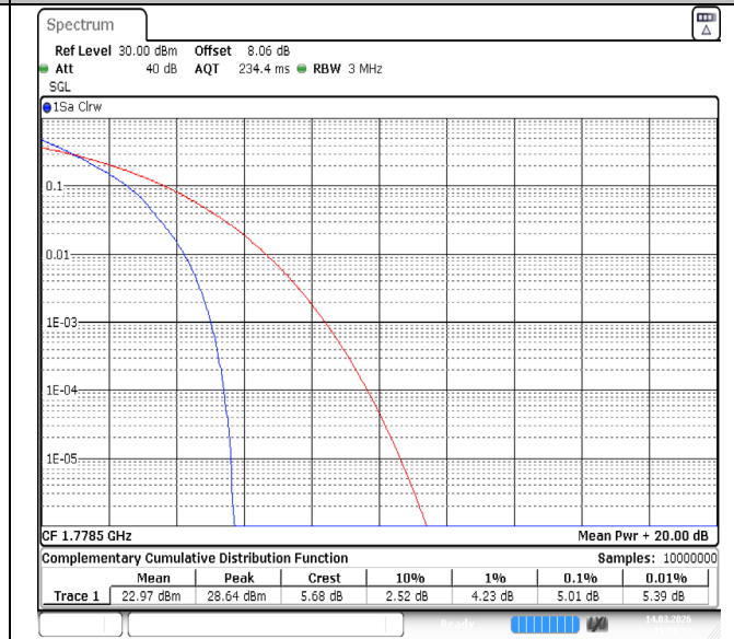
Band66-3MHz-QPSK-132657-15RB#0-PASS
