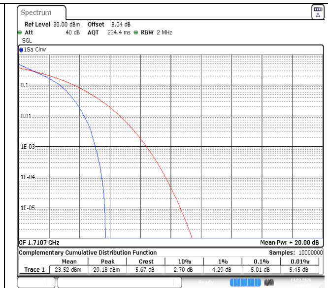
Band66-1.4MHz-QPSK-131979-6RB#0-PASS
