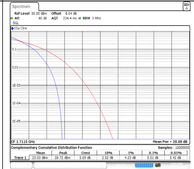
Band66-3MHz-QPSK-131987-15RB#0-PASS
