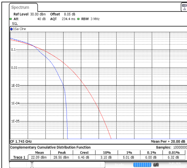
Band66-3MHz-16QAM-132322-1RB#0-PASS
