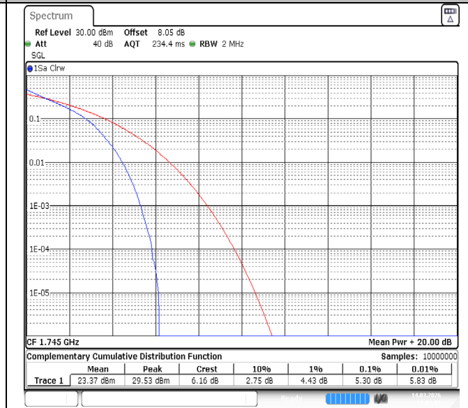
Band66-1.4MHz-QPSK-132322-6RB#0-PASS
