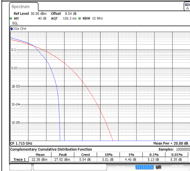
Band66-10MHz-64QAM-132022-1RB#0-PASS
