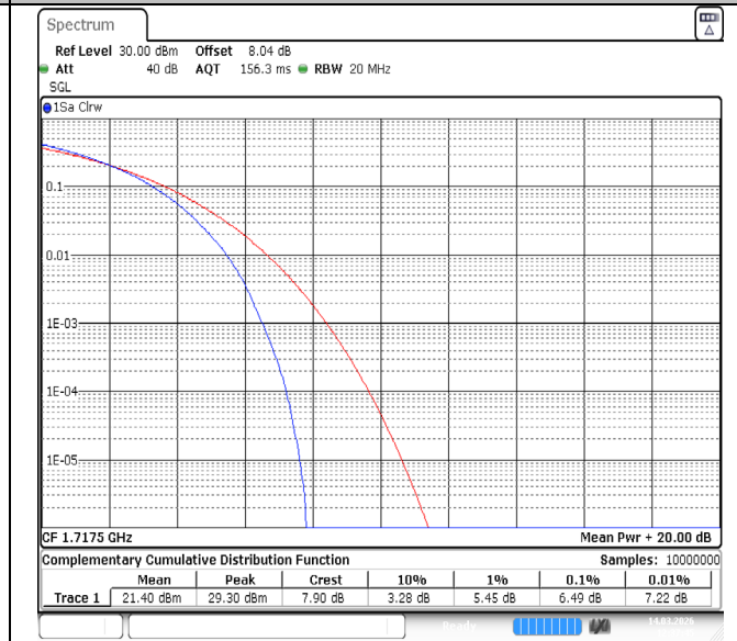
Band66-15MHz-64QAM-132047-75RB#0-PASS
