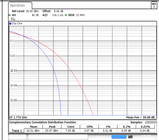
Band66-10MHz-64QAM-132622-50RB#0-PASS
