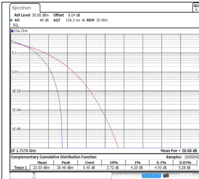
Band66-15MHz-QPSK-132047-1RB#0-PASS
