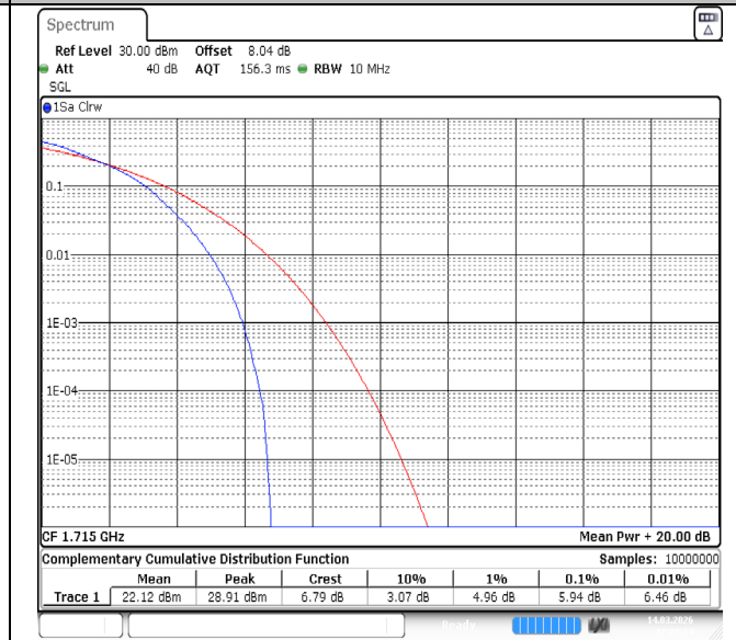
Band66-10MHz-16QAM-132022-50RB#0-PASS
