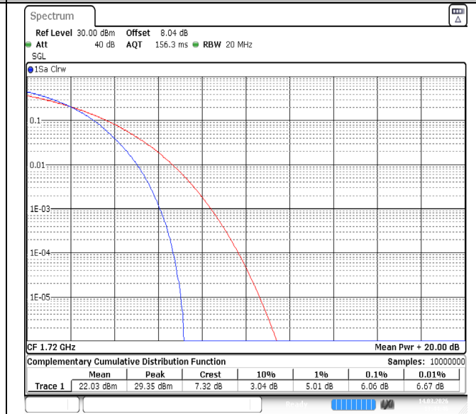
Band66-20MHz-16QAM-132072-100RB#0-PASS
