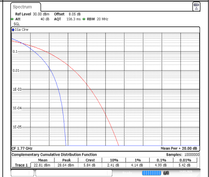
Band66-20MHz-QPSK-132572-100RB#0-PASS
