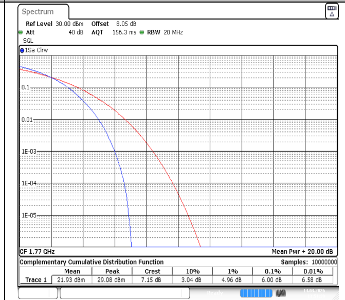
Band66-20MHz-16QAM-132572-100RB#0-PASS
