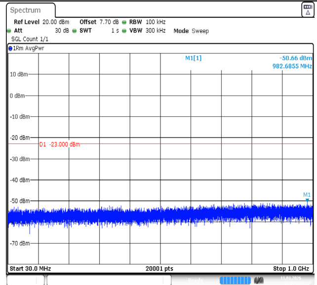
Band4-1.4MHz-QPSK-19957-1RB#5-30~1000-PASS
