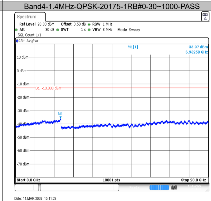
Band4-1.4MHz-QPSK-20175-1RB#0-3000~20000-PASS
