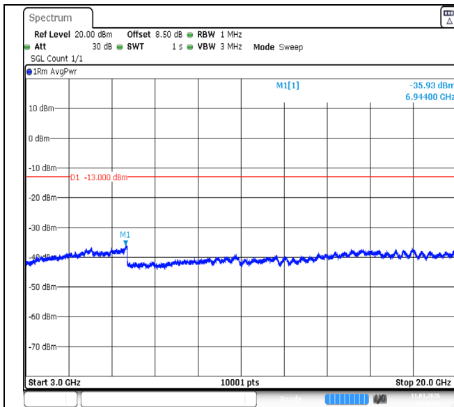
Band4-1.4MHz-QPSK-20393-1RB#0-3000~20000-PASS
