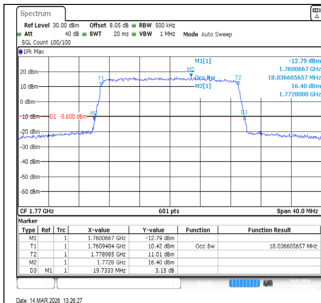
Band66-20MHz-64QAM-132572-100RB#0-PASS
