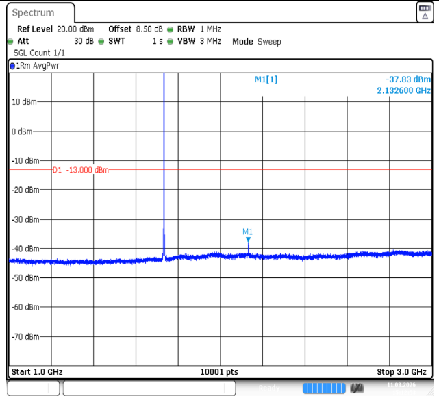
Band4-1.4MHz-QPSK-20175-1RB#5-1000~3000-PASS
