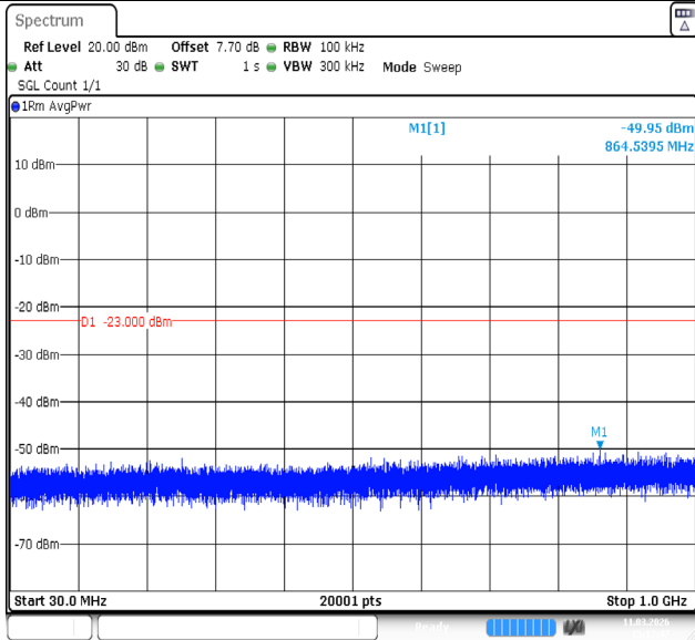
Band4-1.4MHz-QPSK-20175-1RB#5-30~1000-PASS
