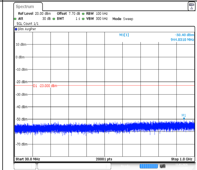
Band4-20MHz-QPSK-20050-1RB#0-30~1000-PASS
