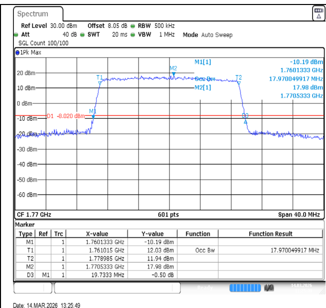
Band66-20MHz-16QAM-132572-100RB#0-PASS
