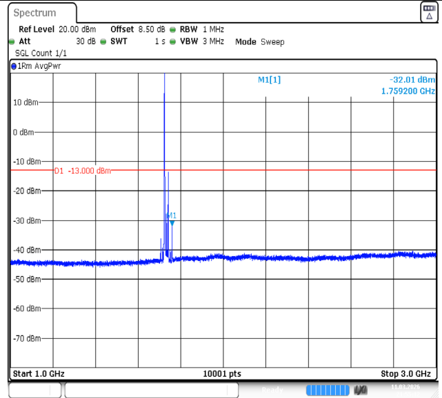
Band4-20MHz-QPSK-20175-1RB#0-1000~3000-PASS
