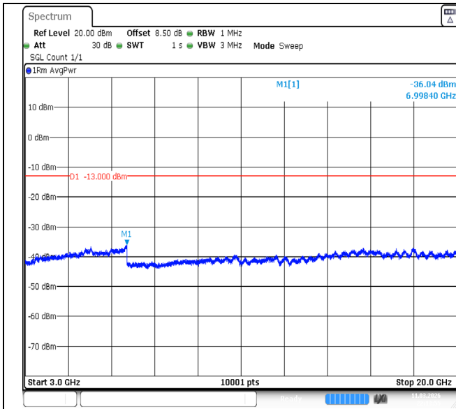
Band4-20MHz-QPSK-20175-100RB#0-3000~20000-PASS
