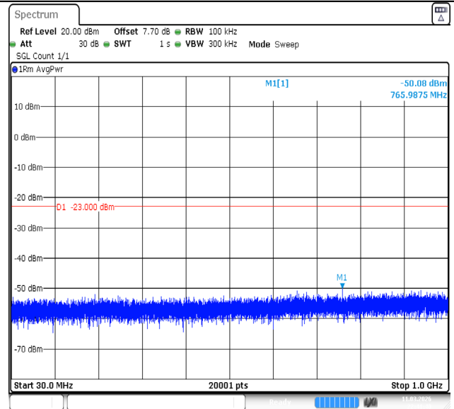
Band4-20MHz-QPSK-20300-100RB#0-30~1000-PASS
