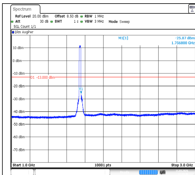
Band4-20MHz-QPSK-20300-100RB#0-1000~3000-PASS
