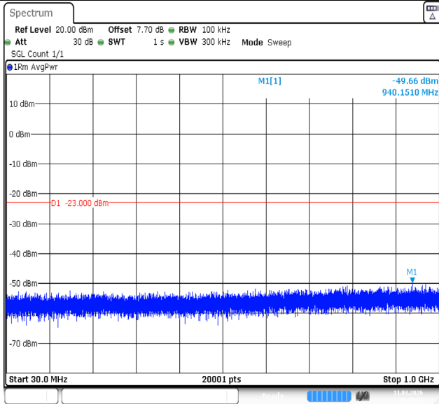
Band4-20MHz-QPSK-20300-1RB#99-30~1000-PASS
