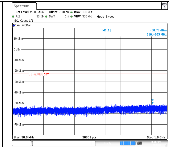
Band4-20MHz-QPSK-20300-1RB#0-30~1000-PASS
