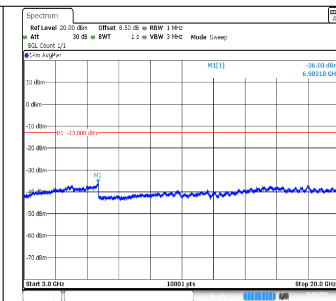
Band4-20MHz-QPSK-20300-100RB#0-3000~20000-PASS
