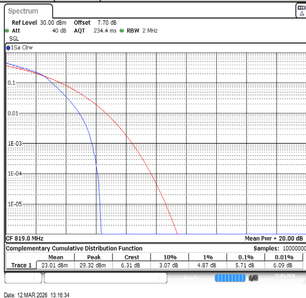
Band26(814-824)-1.4MHz-16QAM-26740-6RB#0-PASS
