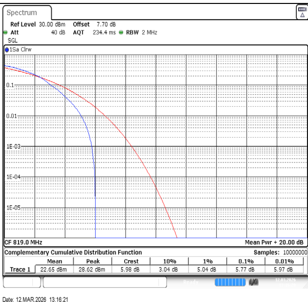
Band26(814-824)-1.4MHz-64QAM-26740-1RB#0-PASS
