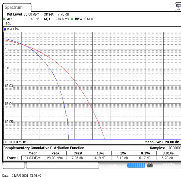
Band26(814-824)-1.4MHz-64QAM-26740-6RB#0-PASS
