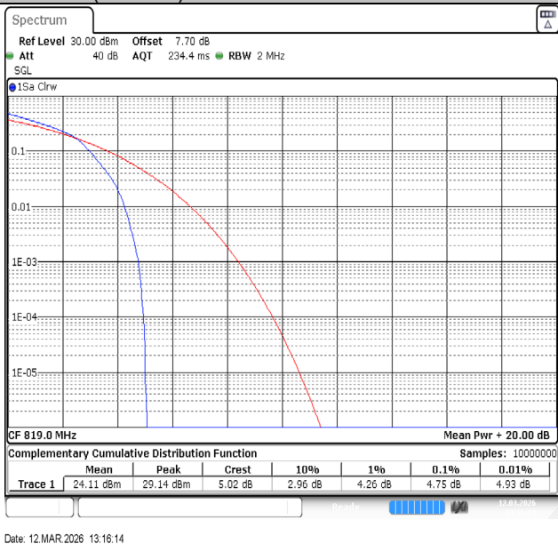
Band26(814-824)-1.4MHz-16QAM-26740-1RB#0-PASS
