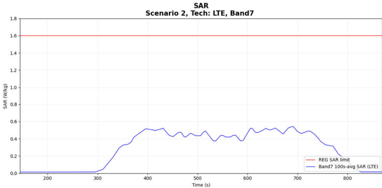
Figure 7-11 Time-averaged SAR
