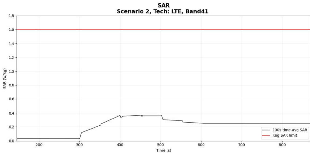
Figure 6- 15 Time-averaged SAR
