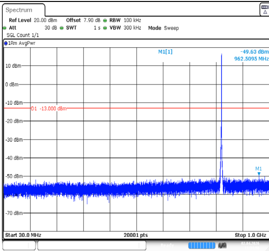
Band26(824-849)-1.4MHz-QPSK-26797-6RB#0-30~1000-PASS
