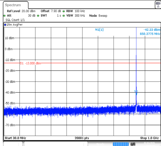
Band26(824-849)-1.4MHz-QPSK-27033-1RB#0-1000~300-PASS
