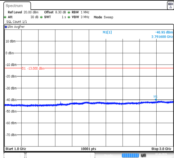
Band5-10MHz-QPSK-20525-1RB#0-1000~3000-PASS
