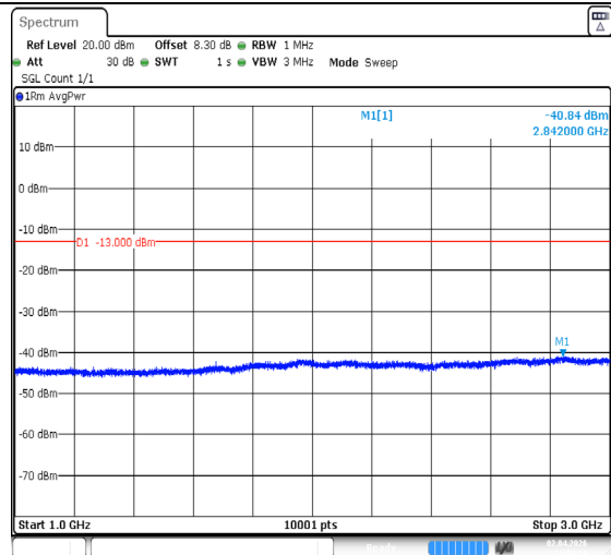
Band26(824-849)-15MHz-QPSK-26865-1RB#74-1000~300 0-PASS
