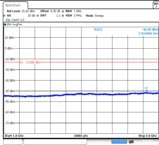
Band26(824-849)-1.4MHz-QPSK-27033-6RB#0-1000~300-PASS
