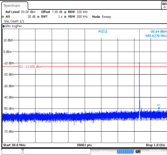
Band26(824-849)-1.4MHz-QPSK-26915-1RB#5-30~1000-PASS
