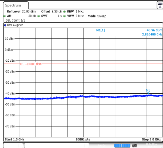
Band26(824-849)-15MHz-QPSK-26915-1RB#0-1000~3000-PASS
