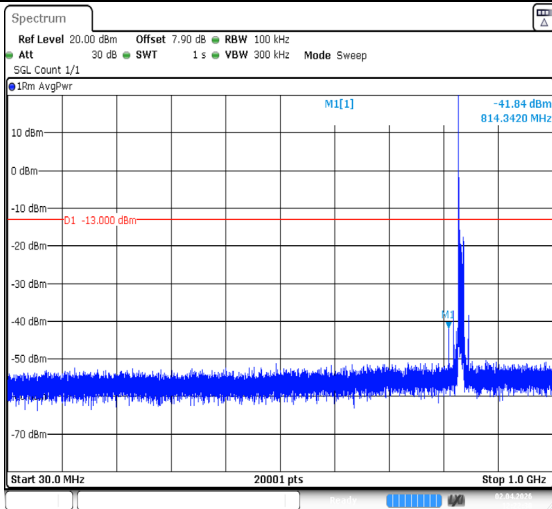
Band5-10MHz-QPSK-20525-1RB#0-30~1000-PASS
