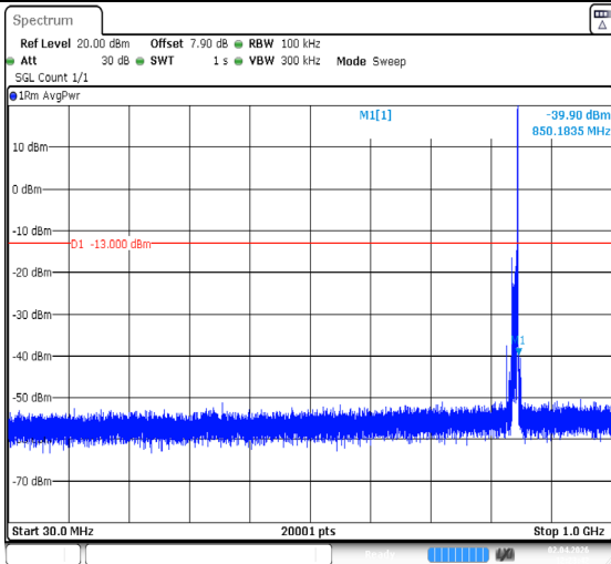
Band5-10MHz-QPSK-20600-1RB#49-30~1000-PASS
