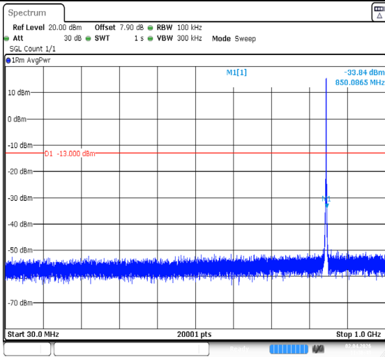
Band26(824-849)-1.4MHz-QPSK-27033-6RB#0-30~1000-PASS
