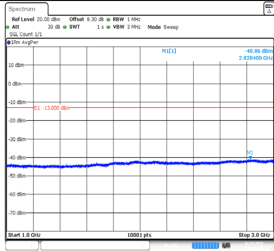
Band26(824-849)-1.4MHz-QPSK-26915-1RB#5-1000~3000-PASS
