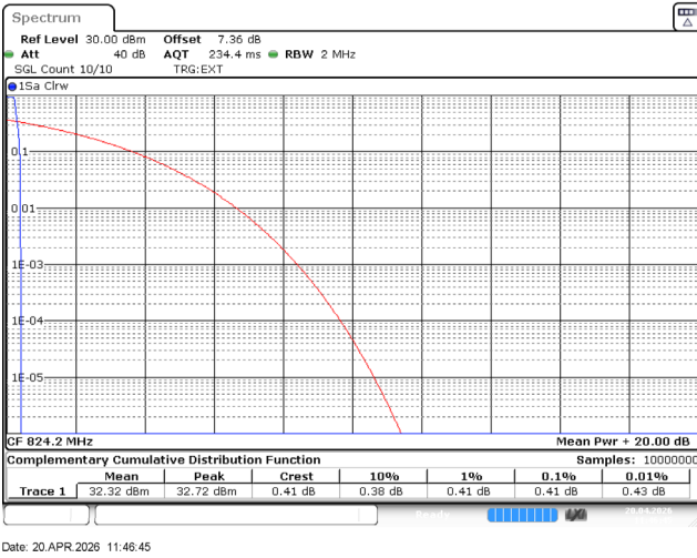
EGPRS850-128-8-PASS
