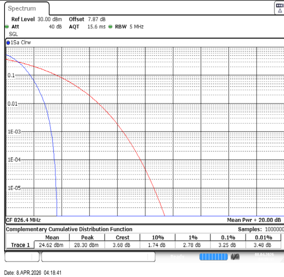
Band5-4132-PASS
