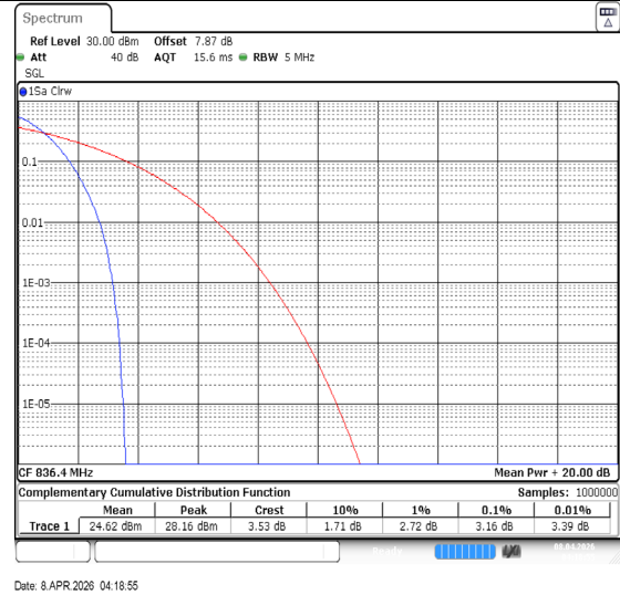
Band5-4182-PASS
