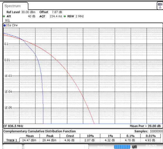
Band5-1.4MHz-64QAM-20525-1RB#0-PASS
