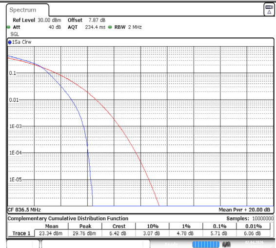
Band5-1.4MHz-64QAM-20525-6RB#0-PASS
