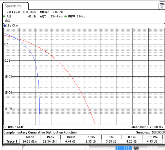
Band5-1.4MHz-QPSK-20525-1RB#0-PASS
