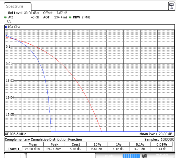
Band5-1.4MHz-QPSK-20525-6RB#0-PASS
