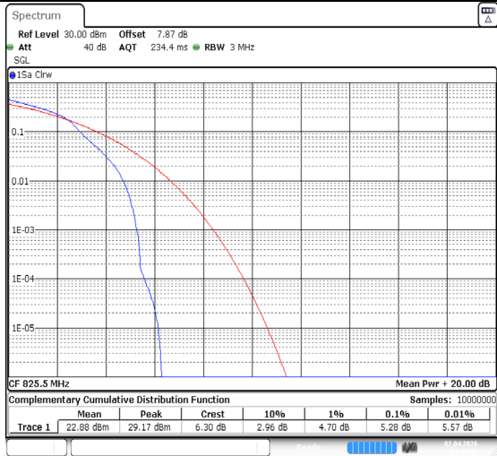
Band26(824-849)-3MHz-64QAM-26805-1RB#0-PASS
