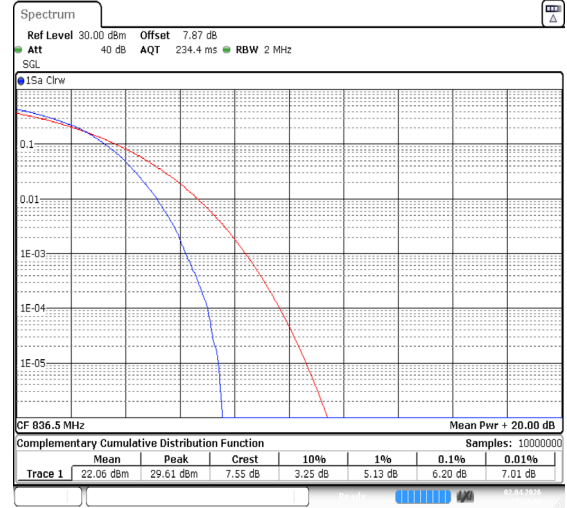
Band26(824-849)-1.4MHz-QPSK-26915-6RB#0-PASS
