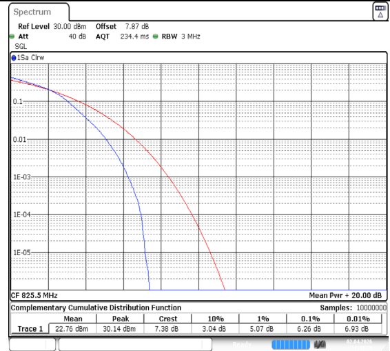
Band26(824-849)-3MHz-64QAM-26805-15RB#0-PASS
