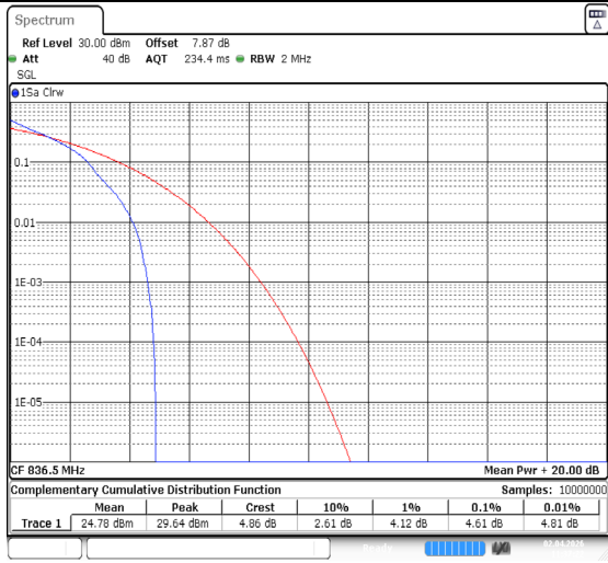
Band26(824-849)-1.4MHz-QPSK-26915-1RB#0-PASS
