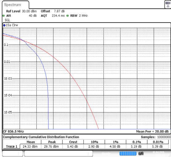
Band26(824-849)-1.4MHz-64QAM-26915-1RB#0-PASS
