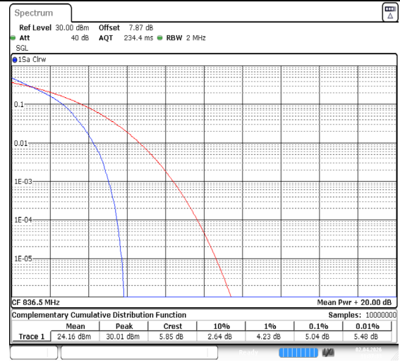
Band26(824-849)-1.4MHz-QPSK-26915-6RB#0-PASS
