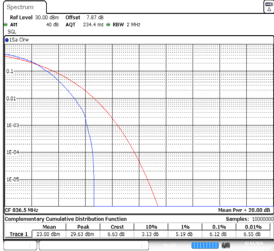
Band26(824-849)-1.4MHz-QPSK-26915-1RB#0-PASS
