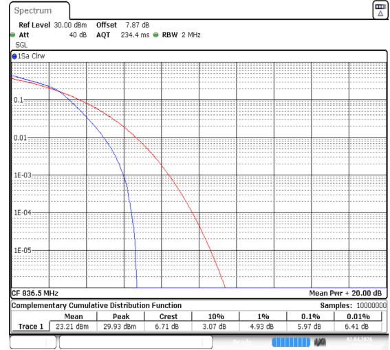
Band26(824-849)-1.4MHz-64QAM-26915-6RB#0-PASS
