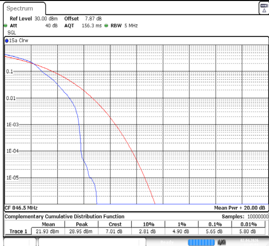
Band26(824-849)-5MHz-64QAM-27015-1RB#0-PASS
