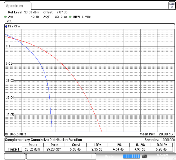
Band26(824-849)-5MHz-QPSK-27015-25RB#0-PASS
