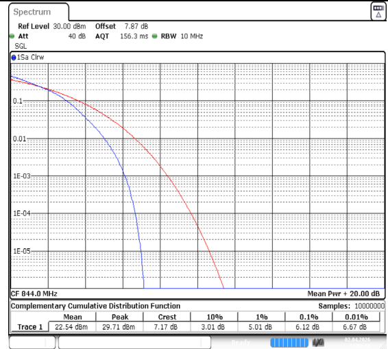
Band26(824-849)-10MHz-64QAM-26990-50RB#0-PASS
