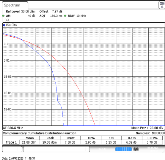
Band26(824-849)-10MHz-16QAM-26915-1RB#0-PASS
