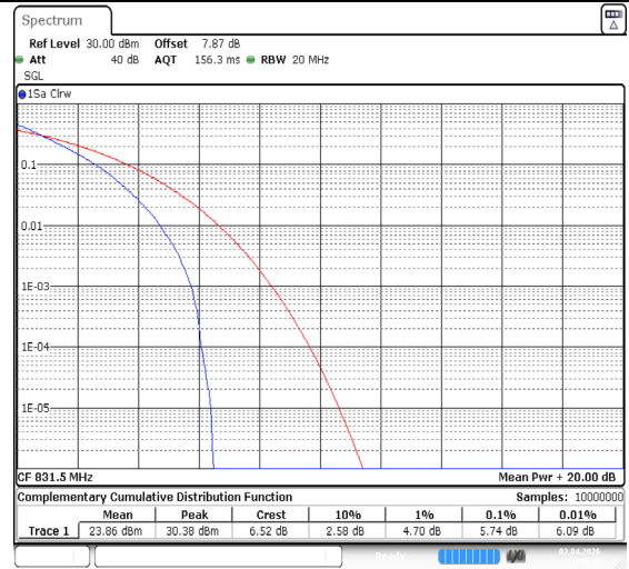
Band26(824-849)-15MHz-QPSK-26865-75RB#0-PASS
