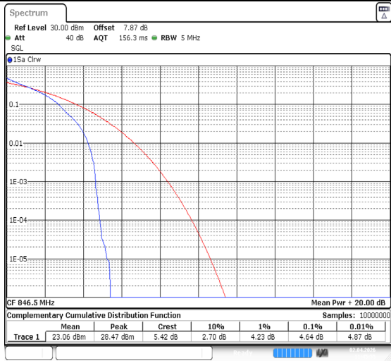
Band26(824-849)-5MHz-QPSK-27015-1RB#0-PASS
