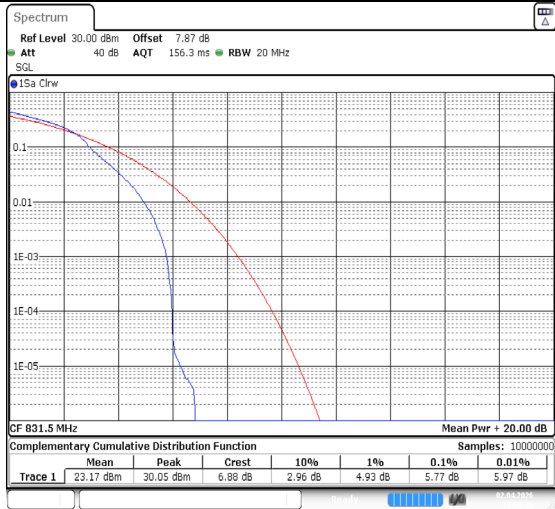
Band26(824-849)-15MHz-64QAM-26865-1RB#0-PASS
