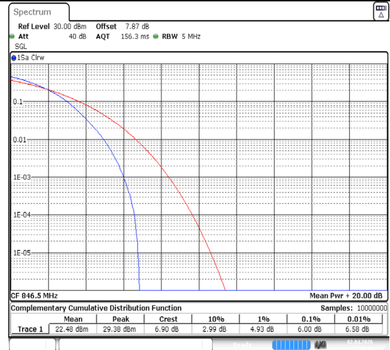
Band26(824-849)-5MHz-64QAM-27015-25RB#0-PASS
