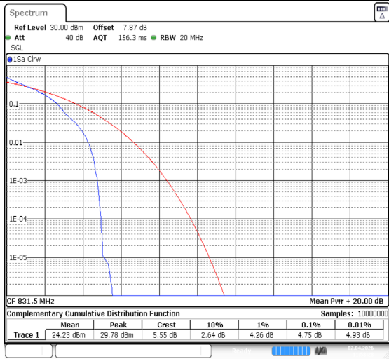
Band26(824-849)-15MHz-QPSK-26865-1RB#0-PASS
