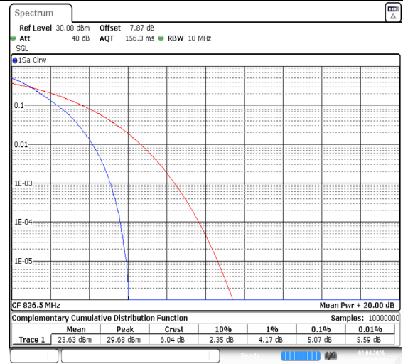
Band26(824-849)-10MHz-QPSK-26915-50RB#0-PASS
