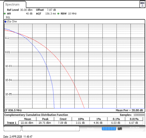
Band26(824-849)-10MHz-16QAM-26915-50RB#0-PASS
