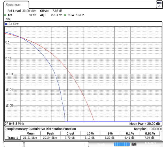
Band26(824-849)-5MHz-QPSK-27015-25RB#0-PASS
