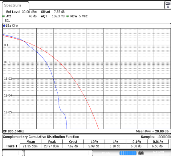
Band26(824-849)-5MHz-64QAM-26915-1RB#0-PASS
