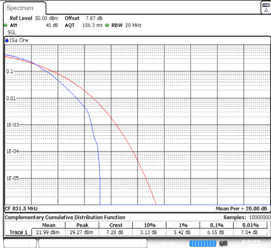
Band26(824-849)-15MHz-QPSK-26865-1RB#0-PASS
