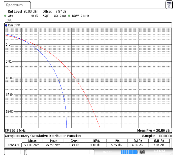
Band26(824-849)-5MHz-QPSK-26915-25RB#0-PASS
