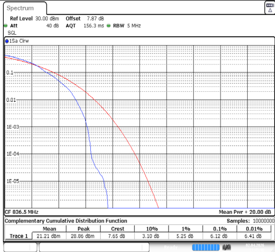
Band26(824-849)-5MHz-QPSK-26915-1RB#0-PASS
