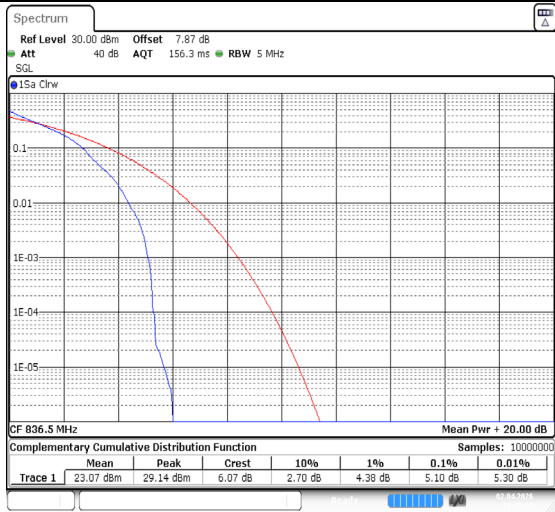
Band26(824-849)-5MHz-QPSK-26915-1RB#0-PASS
