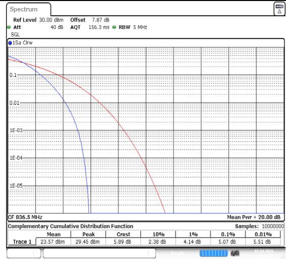
Band26(824-849)-5MHz-QPSK-26915-25RB#0-PASS
