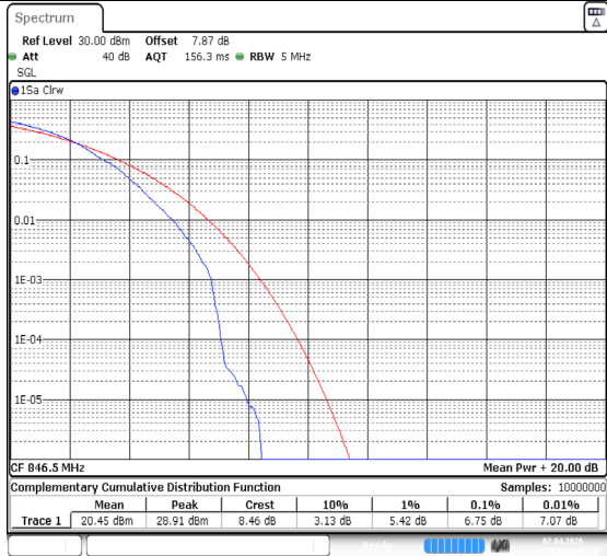
Band26(824-849)-5MHz-QPSK-27015-1RB#0-PASS
