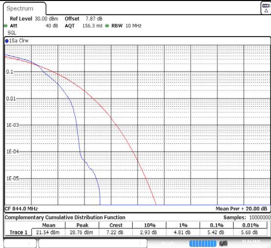
Band26(824-849)-10MHz-64QAM-26990-1RB#0-PASS
