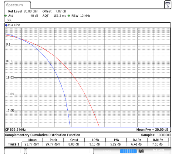
Band26(824-849)-10MHz-QPSK-26915-50RB#0-PASS
