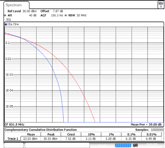
Band26(824-849)-15MHz-64QAM-26865-75RB#0-PASS
