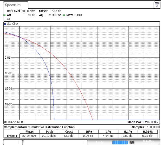
Band26(824-849)-3MHz-64QAM-27025-15RB#0-PASS
