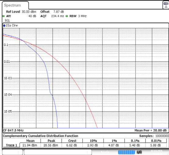
Band26(824-849)-3MHz-64QAM-27025-1RB#0-PASS
