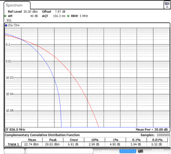
Band26(824-849)-5MHz-64QAM-26915-25RB#0-PASS
