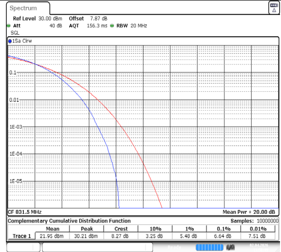
Band26(824-849)-15MHz-QPSK-26865-75RB#0-PASS
