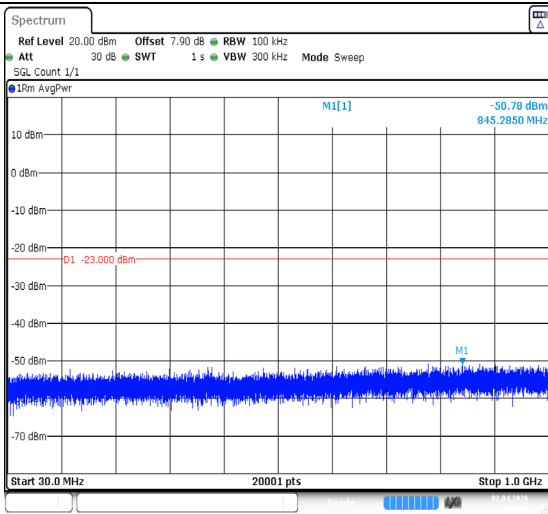
Band2-1.4MHz-QPSK-19193-6RB#0-30~1000-PASS
