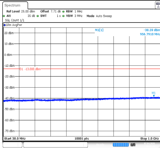
Band2-9262-30~1000MHz-PASS
