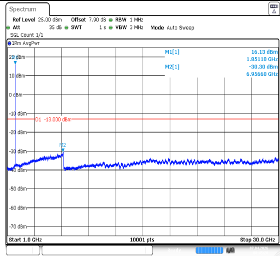
Band2-9262-1000~30000MHz-PASS
