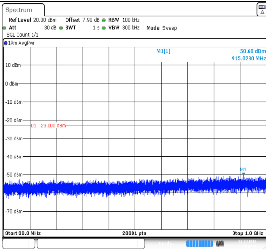
Band2-20MHz-QPSK-18900-1RB#0-30~1000-PASS
