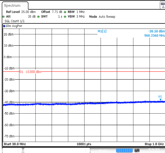
Band2-9538-30~1000MHz-PASS
