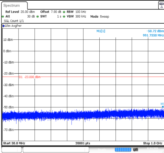
Band2-1.4MHz-QPSK-19193-1RB#0-30~1000-PASS
