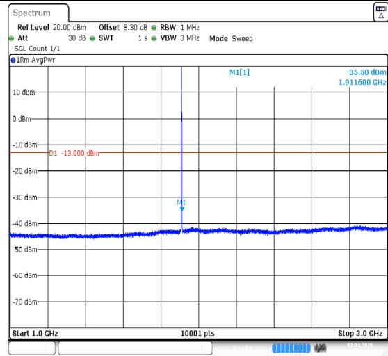
Band2-1.4MHz-QPSK-19193-1RB#0-1000~3000-PASS
