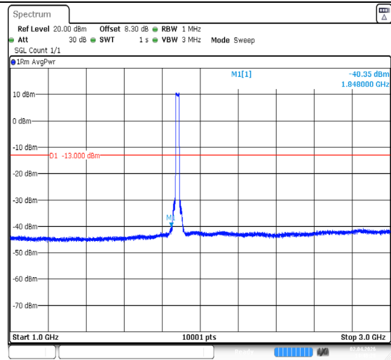
Band2-20MHz-QPSK-18900-100RB#0-1000~3000-PASS
