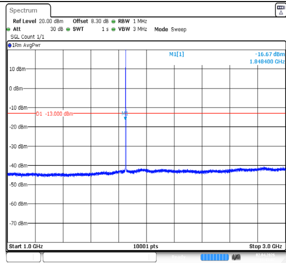
Band2-1.4MHz-QPSK-18607-1RB#0-1000~3000-PASS
