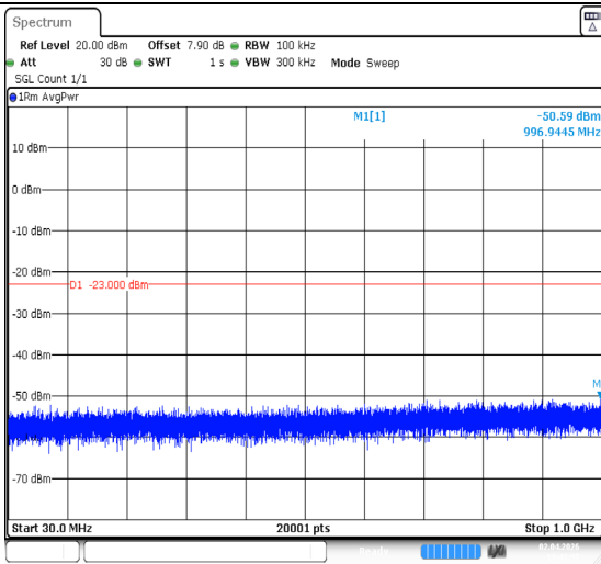
Band2-1.4MHz-QPSK-18607-6RB#0-30~1000-PASS
