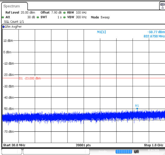
Band2-1.4MHz-QPSK-18900-1RB#5-30~1000-PASS
