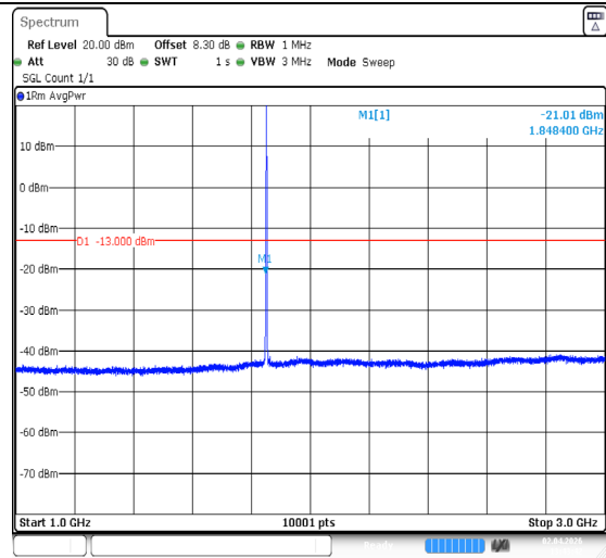
Band2-1.4MHz-QPSK-18607-6RB#0-1000~3000-PASS
