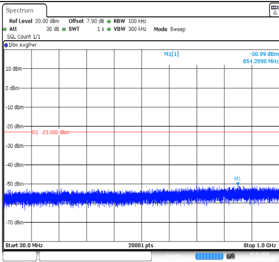
Band2-20MHz-QPSK-18900-100RB#0-30~1000-PASS
