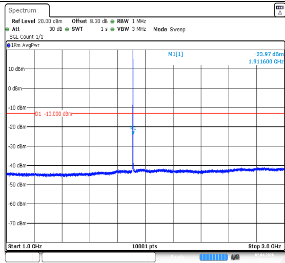
Band2-1.4MHz-QPSK-19193-6RB#0-1000~3000-PASS
