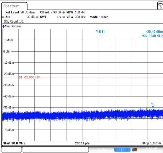
Band2-20MHz-QPSK-18700-1RB#99-30~1000-PASS
