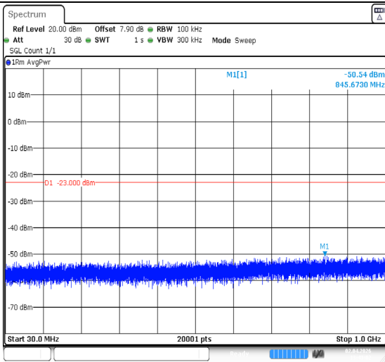
Band2-1.4MHz-QPSK-18607-1RB#0-30~1000-PASS
