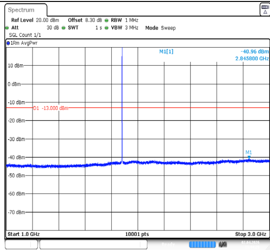
Band2-1.4MHz-QPSK-18900-1RB#5-1000~3000-PASS
