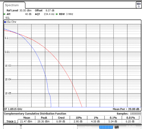
Band2-3MHz-64QAM-18615-15RB#0-PASS
