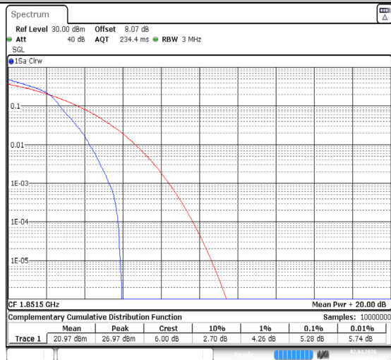
Band2-3MHz-64QAM-18615-1RB#0-PASS
