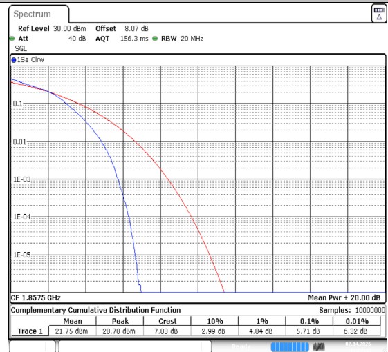
Band2-15MHz-64QAM-18675-75RB#0-PASS
