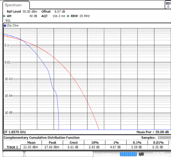
Band2-15MHz-QPSK-18675-1RB#0-PASS
