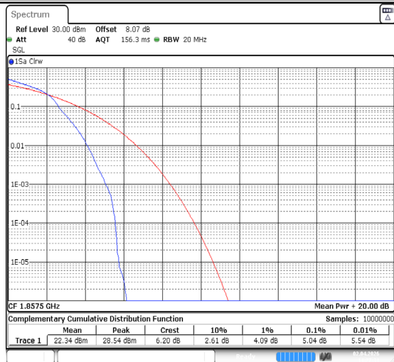
Band2-15MHz-64QAM-18675-1RB#0-PASS
