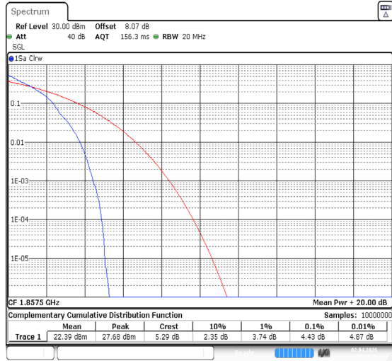
Band2-15MHz-QPSK-18675-1RB#0-PASS
