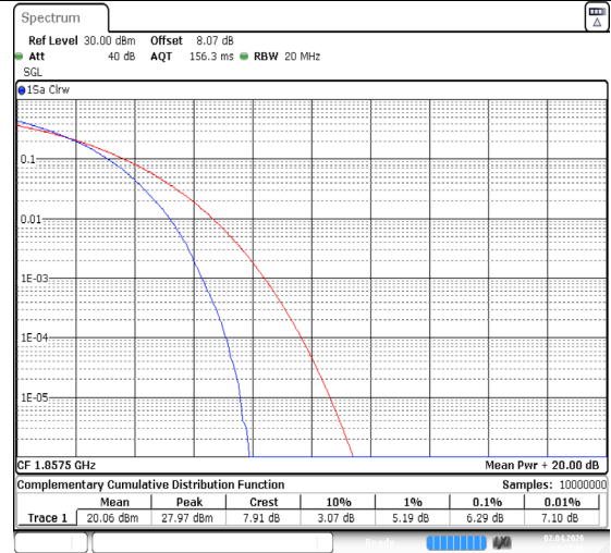
Band2-15MHz-QPSK-18675-75RB#0-PASS
