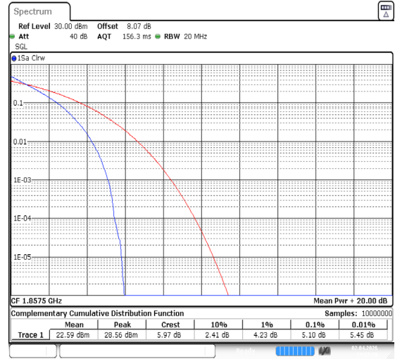
Band2-15MHz-QPSK-18675-75RB#0-PASS
