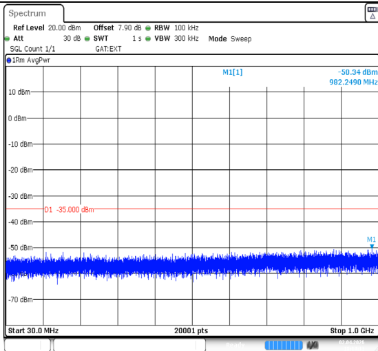
Band41-5MHz-QPSK-40620-1RB#0-30~1000-PASS
