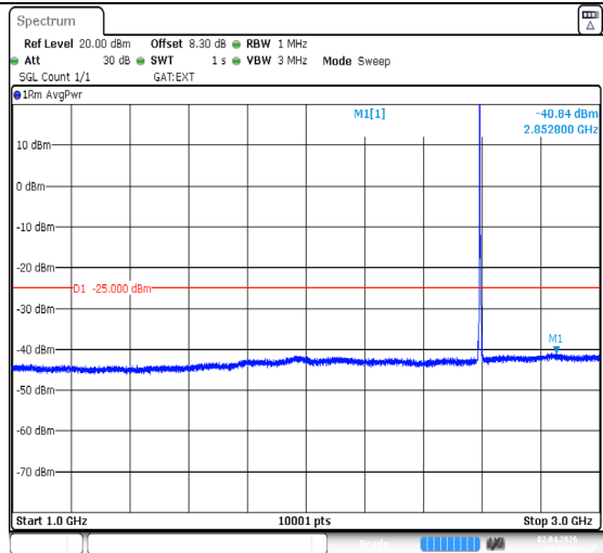
Band41-5MHz-QPSK-40620-1RB#0-1000~3000-PASS
