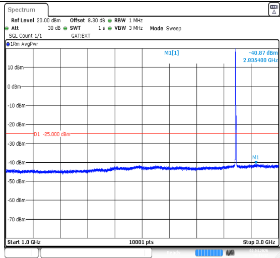
Band41-5MHz-QPSK-41565-1RB#0-1000~3000-PASS
