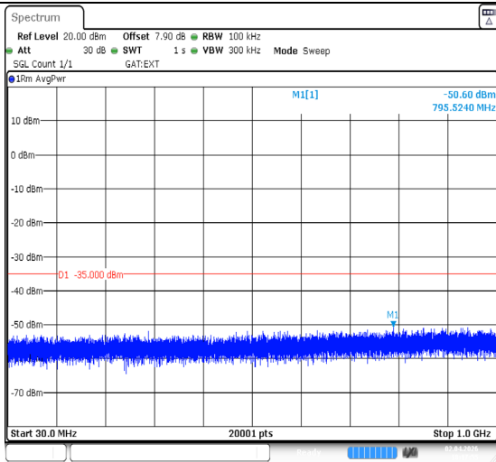
Band41-5MHz-QPSK-41565-1RB#0-30~1000-PASS
