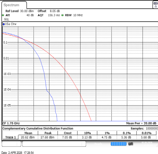
Band4-10MHz-64QAM-20350-1RB#0-PASS
