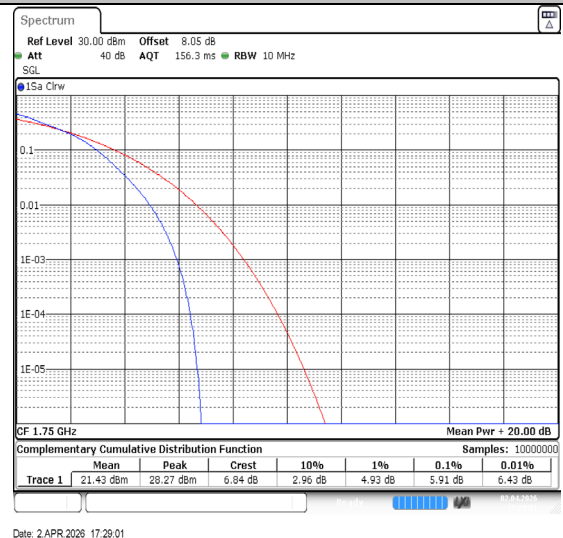
Band4-10MHz-16QAM-20350-50RB#0-PASS
