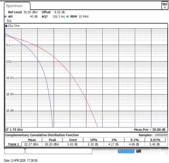
Band4-10MHz-QPSK-20350-50RB#0-PASS
