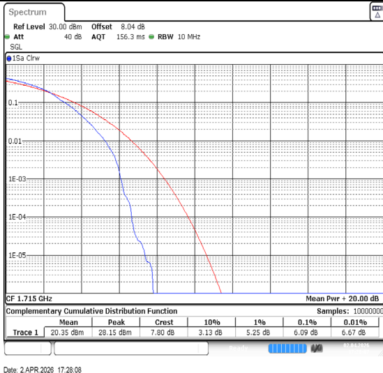
Band4-10MHz-64QAM-20000-1RB#0-PASS
