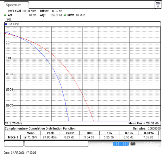
Band4-10MHz-64QAM-20350-50RB#0-PASS
