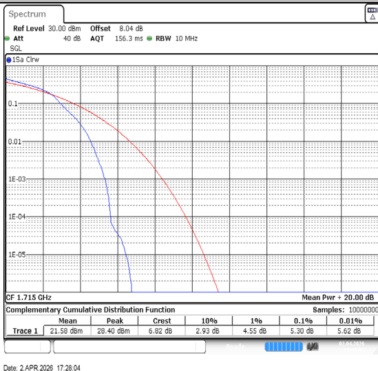
Band4-10MHz-16QAM-20000-1RB#0-PASS
