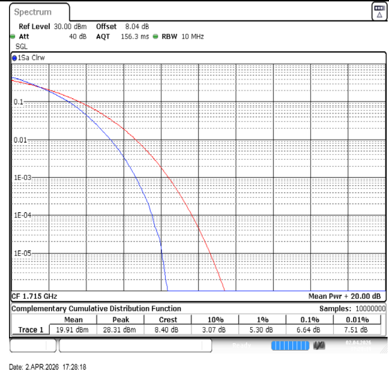
Band4-10MHz-64QAM-20000-50RB#0-PASS
