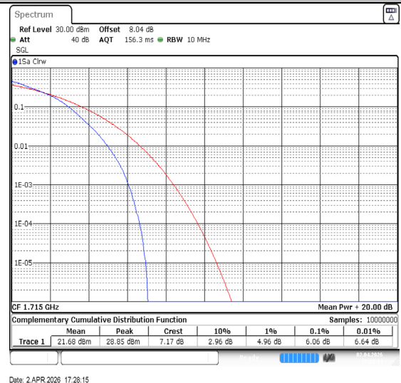
Band4-10MHz-16QAM-20000-50RB#0-PASS
