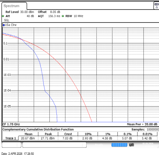
Band4-10MHz-16QAM-20350-1RB#0-PASS
