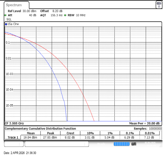
Band7-10MHz-64QAM-20800-50RB#0-PASS
