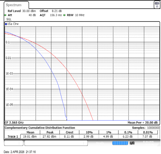
Band7-10MHz-64QAM-21400-50RB#0-PASS
