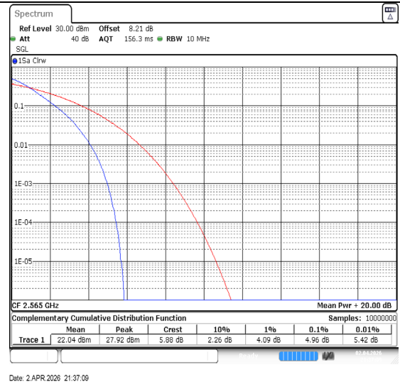
Band7-10MHz-QPSK-21400-50RB#0-PASS
