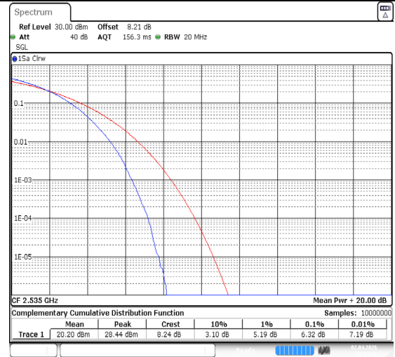
Band7-15MHz-QPSK-21100-75RB#0-PASS
