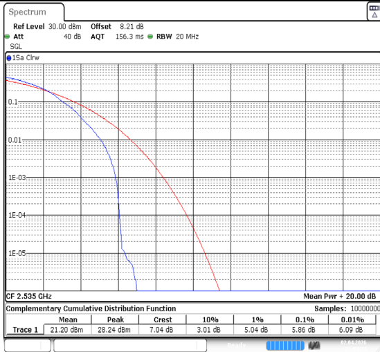
Band7-15MHz-QPSK-21100-1RB#0-PASS
