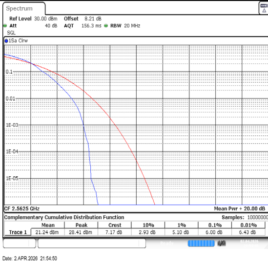
Band7-15MHz-64QAM-21375-1RB#0-PASS
