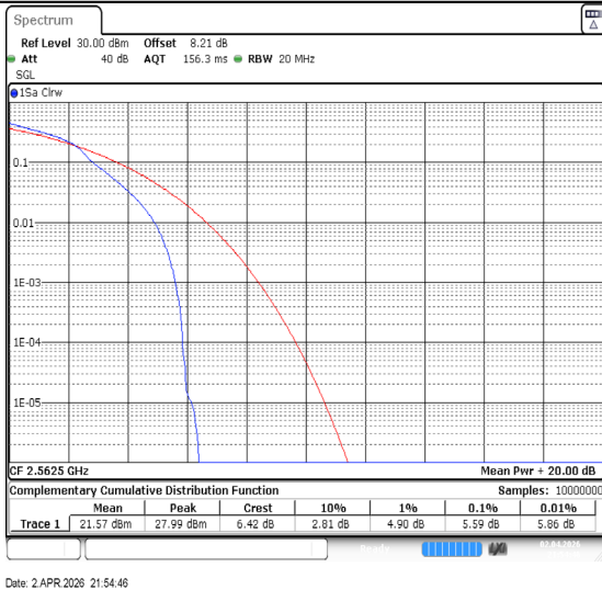
Band7-15MHz-16QAM-21375-1RB#0-PASS
