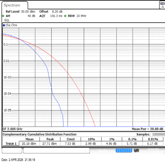
Band7-10MHz-64QAM-20800-1RB#0-PASS
