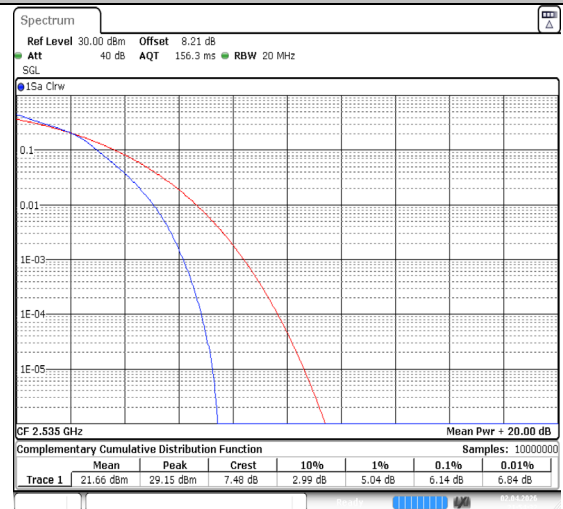
Band7-15MHz-64QAM-21100-75RB#0-PASS
