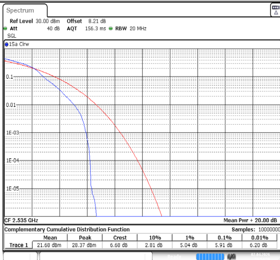
Band7-15MHz-64QAM-21100-1RB#0-PASS
