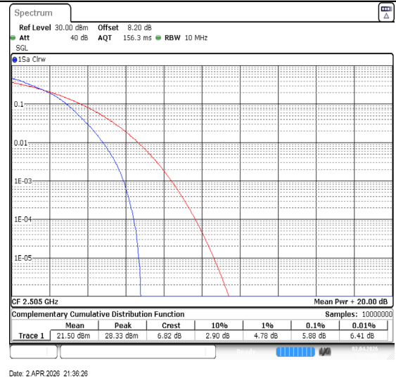
Band7-10MHz-16QAM-20800-50RB#0-PASS
