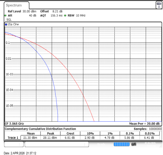
Band7-10MHz-16QAM-21400-50RB#0-PASS
