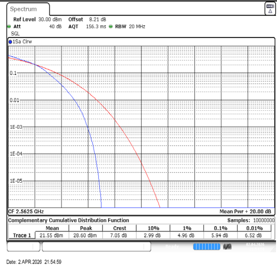
Band7-15MHz-16QAM-21375-75RB#0-PASS
