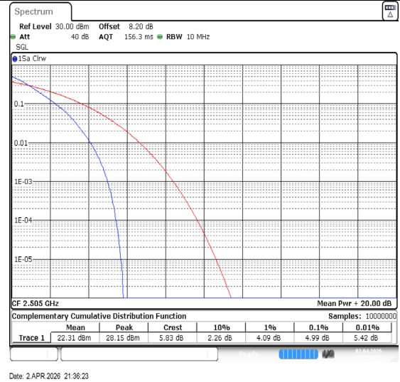
Band7-10MHz-QPSK-20800-50RB#0-PASS
