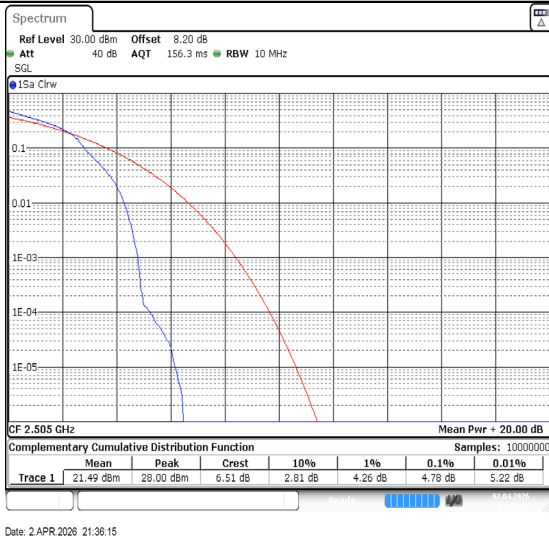
Band7-10MHz-16QAM-20800-1RB#0-PASS
