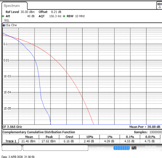
Band7-10MHz-QPSK-21400-1RB#0-PASS
