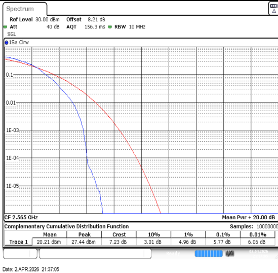
Band7-10MHz-64QAM-21400-1RB#0-PASS
