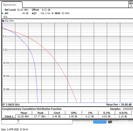
Band7-15MHz-QPSK-21375-1RB#0-PASS
