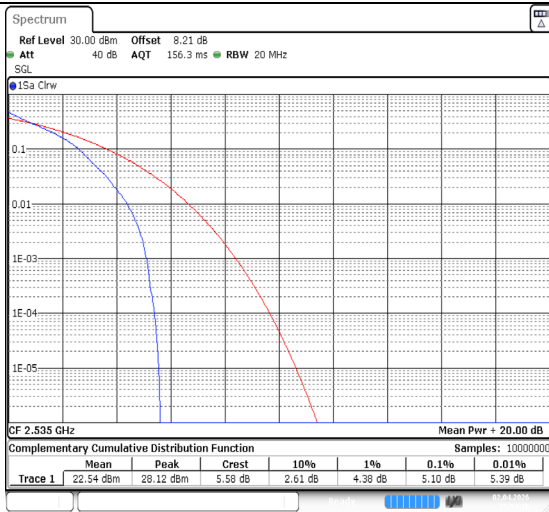
Band7-15MHz-QPSK-21100-1RB#0-PASS
