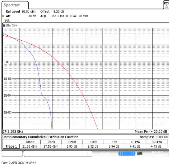
Band7-10MHz-QPSK-20800-1RB#0-PASS
