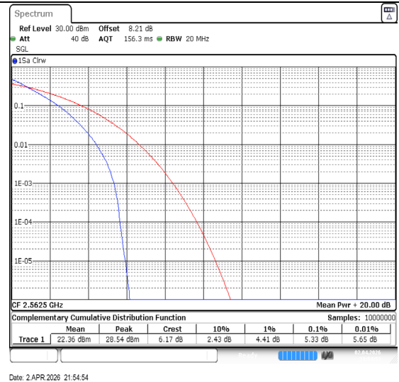
Band7-15MHz-QPSK-21375-75RB#0-PASS
