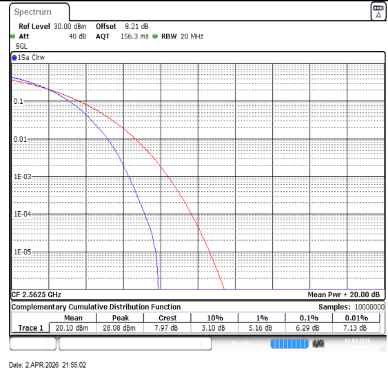
Band7-15MHz-64QAM-21375-75RB#0-PASS
