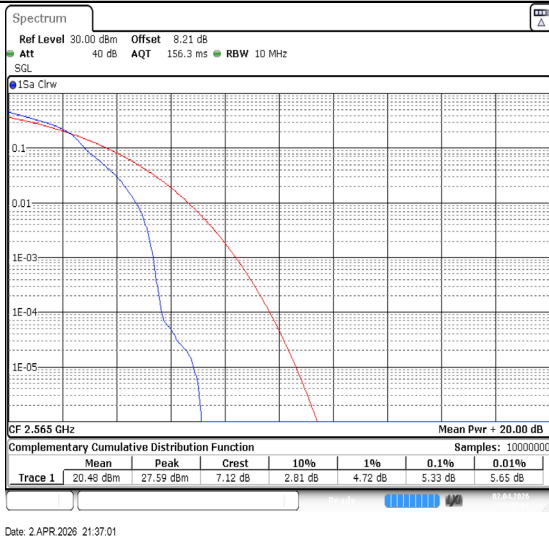
Band7-10MHz-16QAM-21400-1RB#0-PASS
