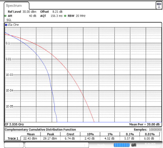
Band7-15MHz-QPSK-21100-75RB#0-PASS
