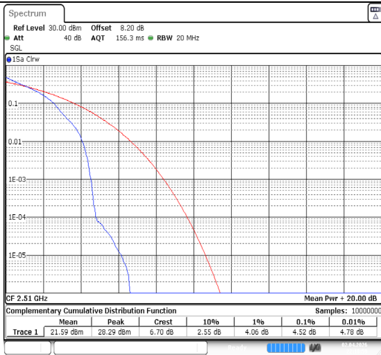
Band7-20MHz-QPSK-20850-1RB#0-PASS
