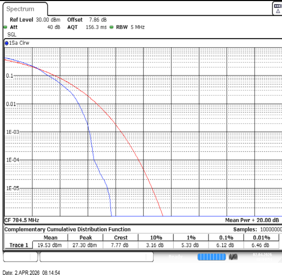
Band13-5MHz-64QAM-23255-1RB#0-PASS
