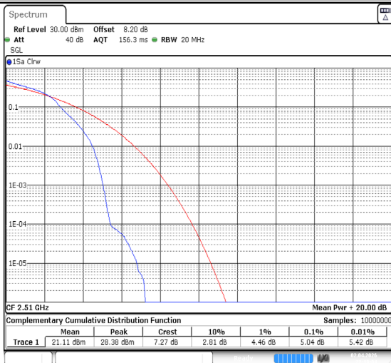
Band7-20MHz-64QAM-20850-1RB#0-PASS
