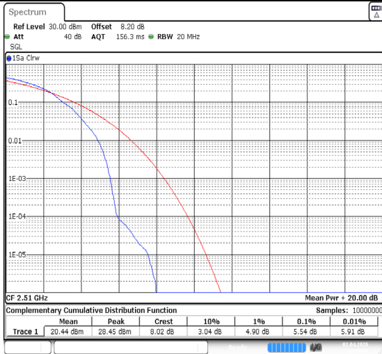
Band7-20MHz-QPSK-20850-1RB#0-PASS
