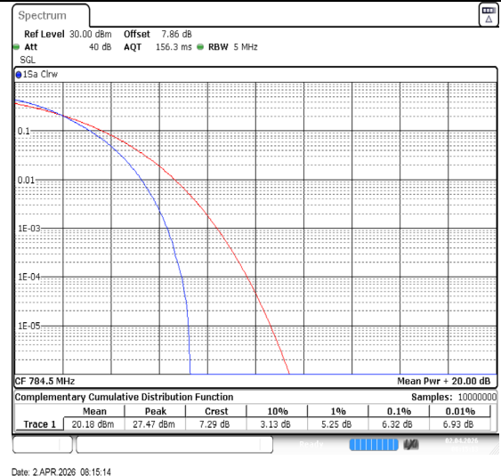
Band13-5MHz-64QAM-23255-25RB#0-PASS
