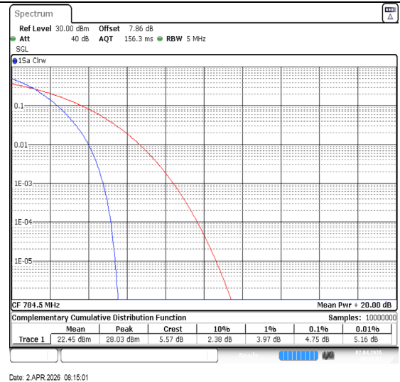
Band13-5MHz-QPSK-23255-25RB#0-PASS
