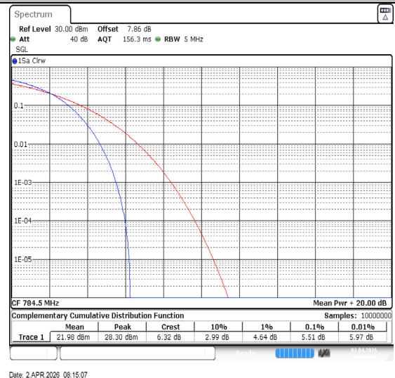
Band13-5MHz-16QAM-23255-25RB#0-PASS
