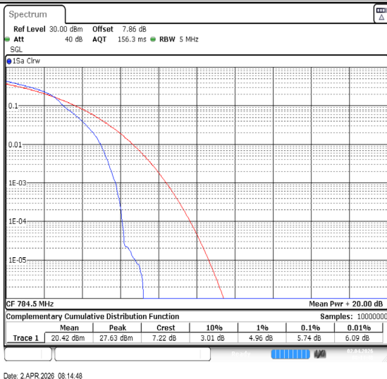
Band13-5MHz-16QAM-23255-1RB#0-PASS
