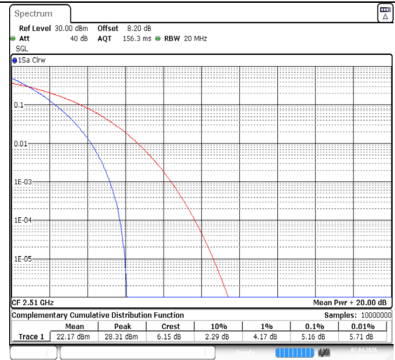
Band7-20MHz-QPSK-20850-100RB#0-PASS
