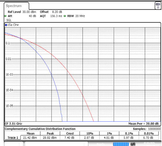
Band7-20MHz-64QAM-20850-100RB#0-PASS
