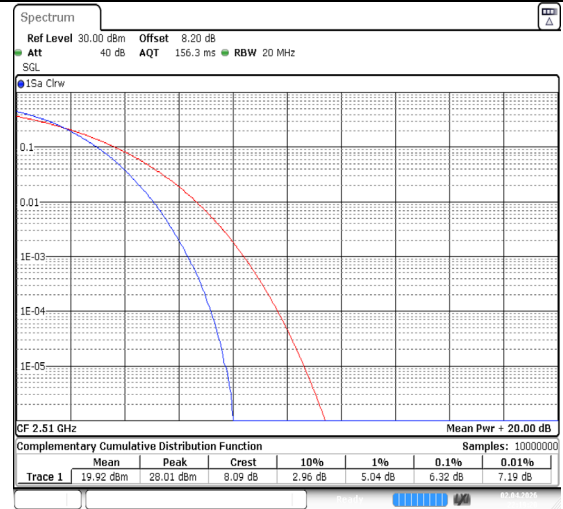
Band7-20MHz-QPSK-20850-100RB#0-PASS
