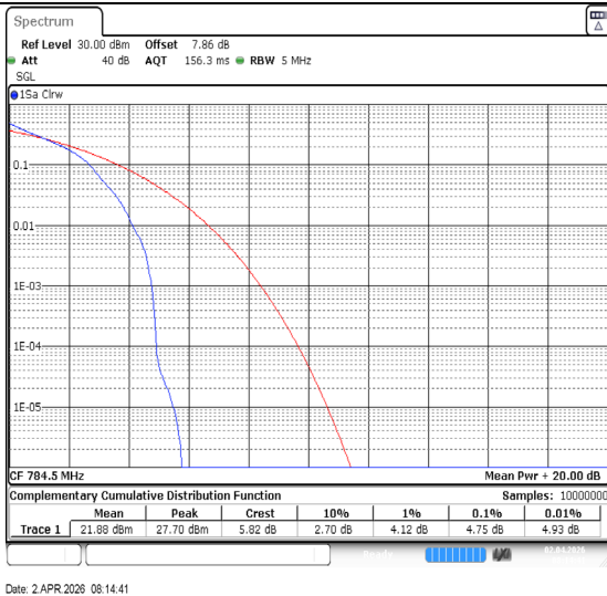
Band13-5MHz-QPSK-23255-1RB#0-PASS
