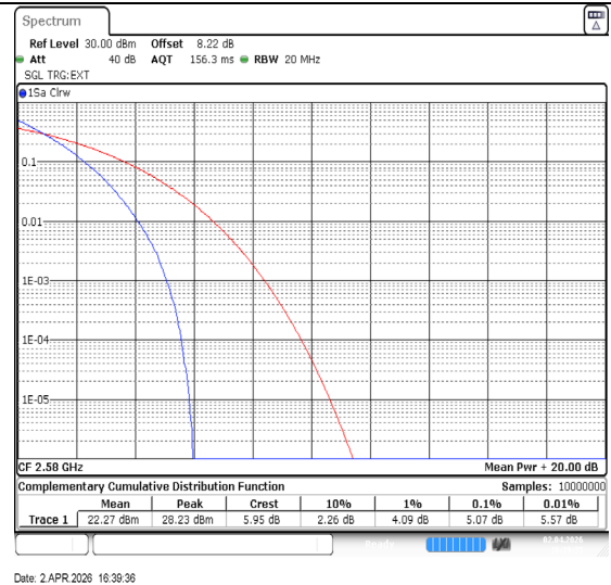
Band38-20MHz-QPSK-37850-100RB#0-PASS
