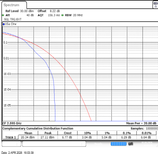
Band38-15MHz-64QAM-38000-1RB#0-PASS
