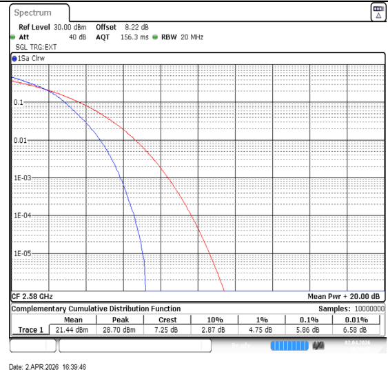
Band38-20MHz-16QAM-37850-100RB#0-PASS
