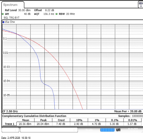
Band38-20MHz-16QAM-37850-1RB#0-PASS
