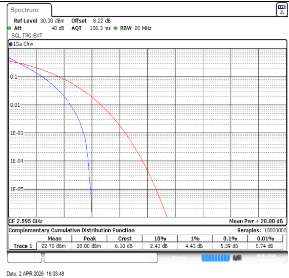
Band38-15MHz-QPSK-38000-75RB#0-PASS
