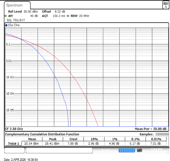
Band38-20MHz-64QAM-37850-100RB#0-PASS
