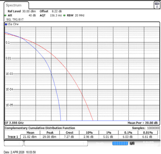
Band38-15MHz-16QAM-38000-75RB#0-PASS
