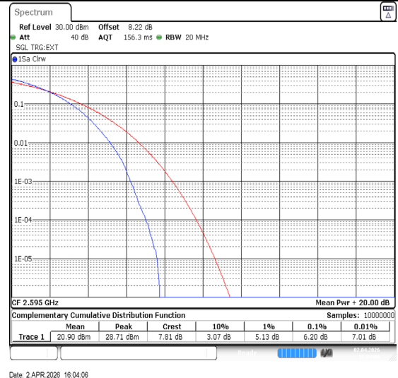
Band38-15MHz-64QAM-38000-75RB#0-PASS
