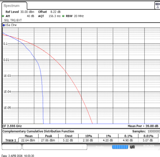
Band38-15MHz-QPSK-38000-1RB#0-PASS
