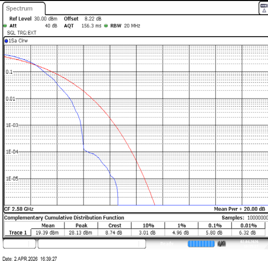
Band38-20MHz-64QAM-37850-1RB#0-PASS
