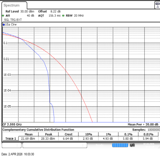
Band38-15MHz-16QAM-38000-1RB#0-PASS
