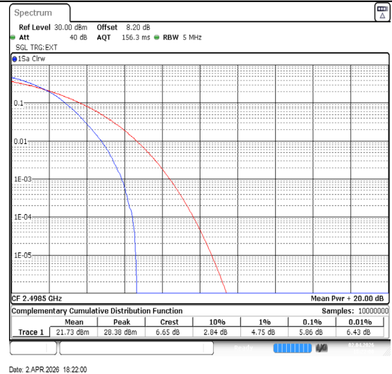
Band41-5MHz-16QAM-39675-25RB#0-PASS
