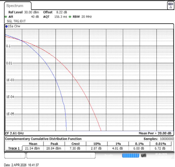
Band38-20MHz-16QAM-38150-100RB#0-PASS
