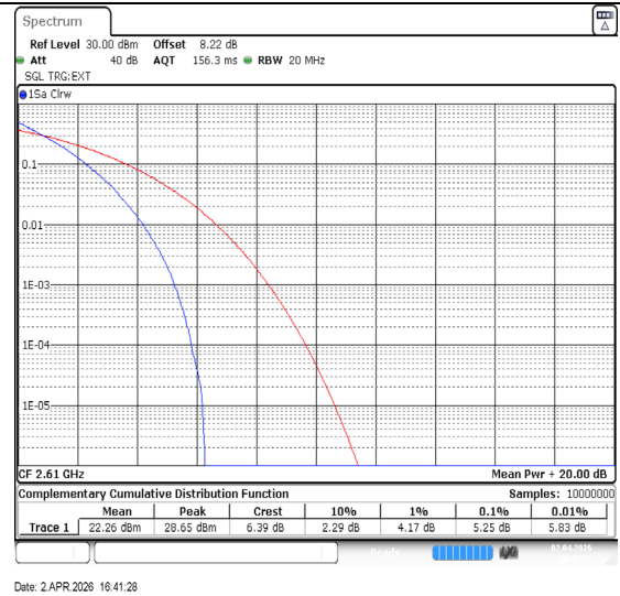
Band38-20MHz-QPSK-38150-100RB#0-PASS
