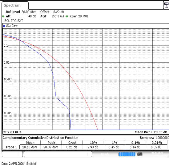
Band38-20MHz-64QAM-38150-1RB#0-PASS
