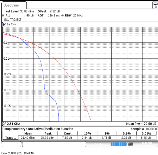
Band38-20MHz-16QAM-38150-1RB#0-PASS
