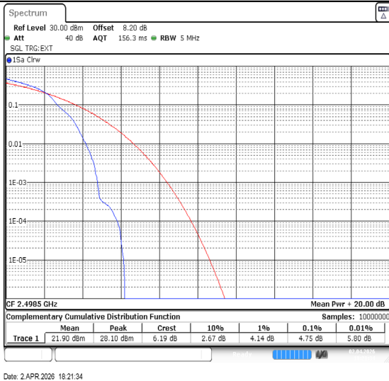
Band41-5MHz-16QAM-39675-1RB#0-PASS
