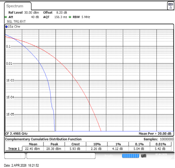
Band41-5MHz-QPSK-39675-25RB#0-PASS
