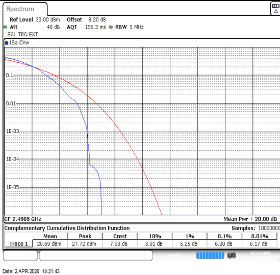
Band41-5MHz-64QAM-39675-1RB#0-PASS
