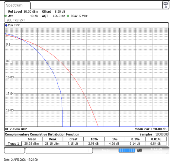
Band41-5MHz-64QAM-39675-25RB#0-PASS
