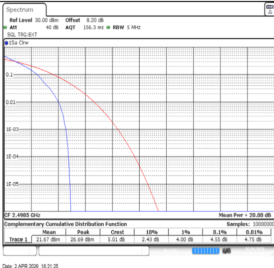
Band41-5MHz-QPSK-39675-1RB#0-PASS
