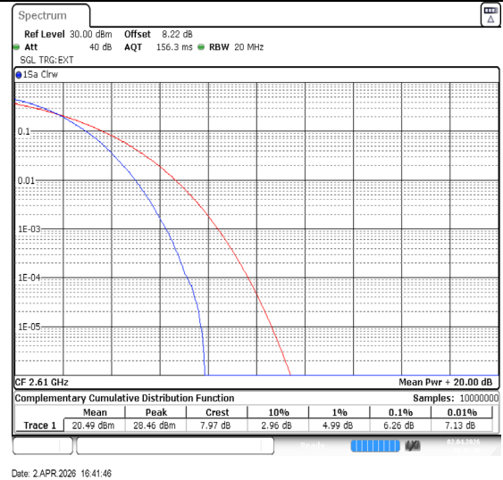
Band38-20MHz-64QAM-38150-100RB#0-PASS
