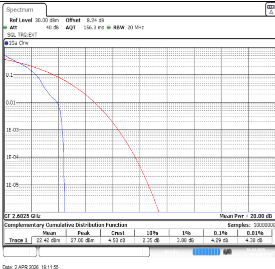
Band41-15MHz-QPSK-41515-1RB#0-PASS
