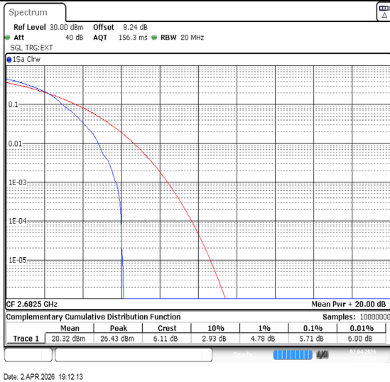
Band41-15MHz-64QAM-41515-1RB#0-PASS
