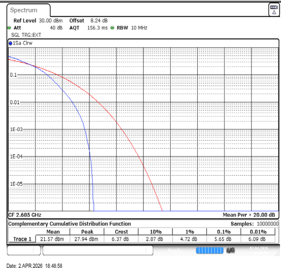
Band41-10MHz-16QAM-41540-50RB#0-PASS
