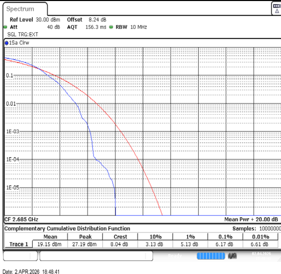
Band41-10MHz-64QAM-41540-1RB#0-PASS
