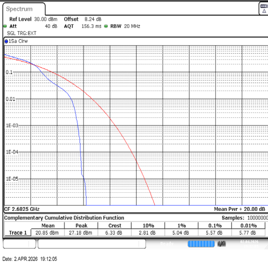
Band41-15MHz-16QAM-41515-1RB#0-PASS
