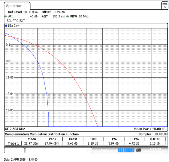
Band41-10MHz-QPSK-41540-50RB#0-PASS
