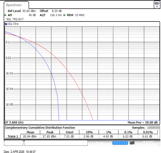
Band41-10MHz-64QAM-41540-50RB#0-PASS
