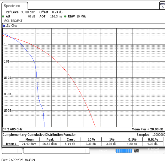
Band41-10MHz-QPSK-41540-1RB#0-PASS
