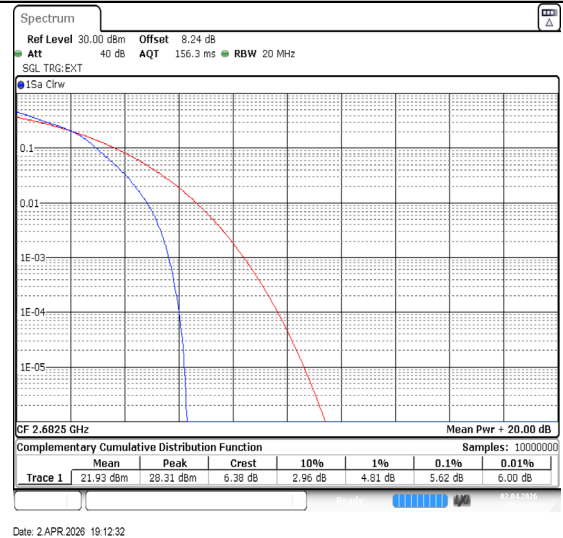
Band41-15MHz-16QAM-41515-75RB#0-PASS
