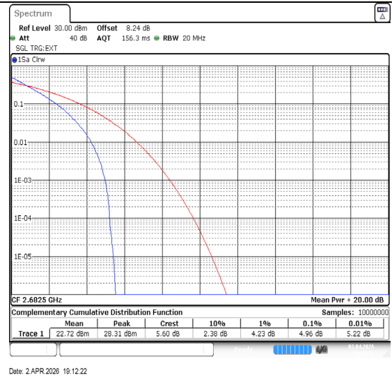
Band41-15MHz-QPSK-41515-75RB#0-PASS
