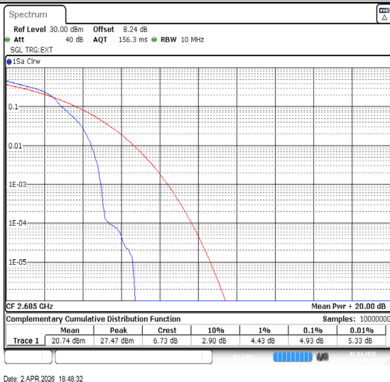
Band41-10MHz-16QAM-41540-1RB#0-PASS
