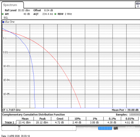
Band66-1.4MHz-QPSK-131979-1RB#0-PASS
