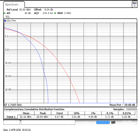
Band66-1.4MHz-16QAM-131979-6RB#0-PASS
