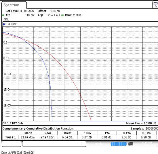
Band66-1.4MHz-64QAM-131979-1RB#0-PASS
