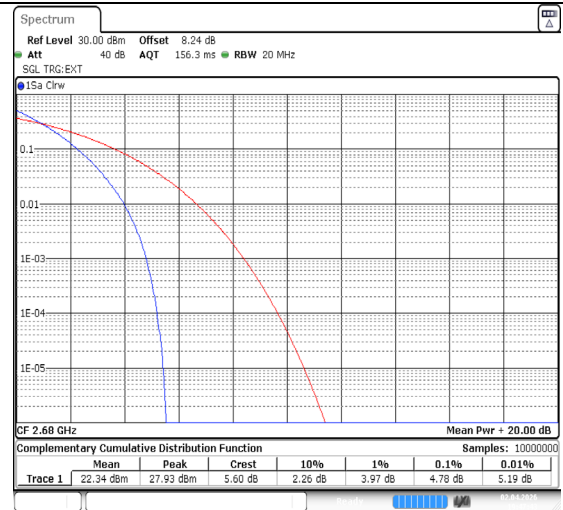
Band41-20MHz-QPSK-41490-100RB#0-PASS
