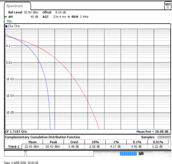
Band66-1.4MHz-QPSK-131979-6RB#0-PASS
