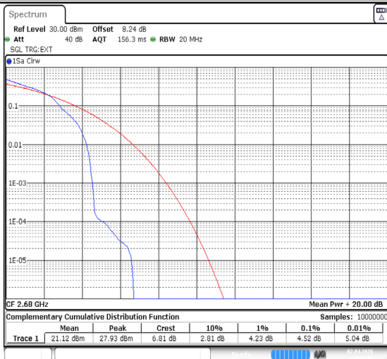
Band41-20MHz-64QAM-41490-1RB#0-PASS
