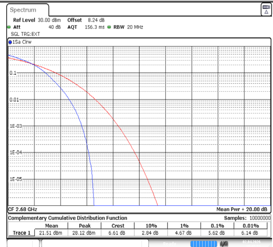
Band41-20MHz-64QAM-41490-100RB#0-PASS
