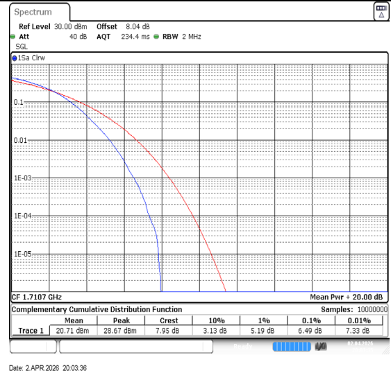
Band66-1.4MHz-64QAM-131979-6RB#0-PASS
