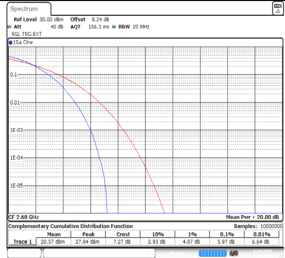
Band41-20MHz-QPSK-41490-100RB#0-PASS
