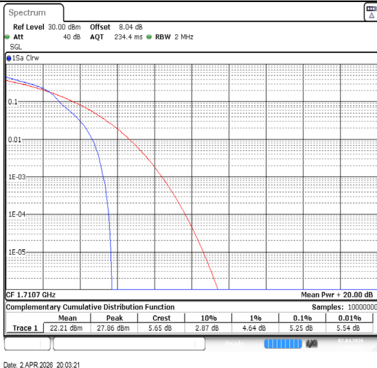
Band66-1.4MHz-16QAM-131979-1RB#0-PASS
