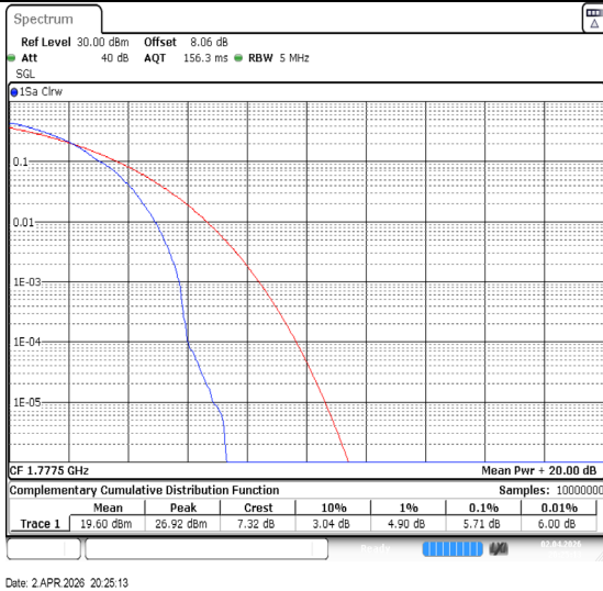
Band66-5MHz-64QAM-132647-1RB#0-PASS
