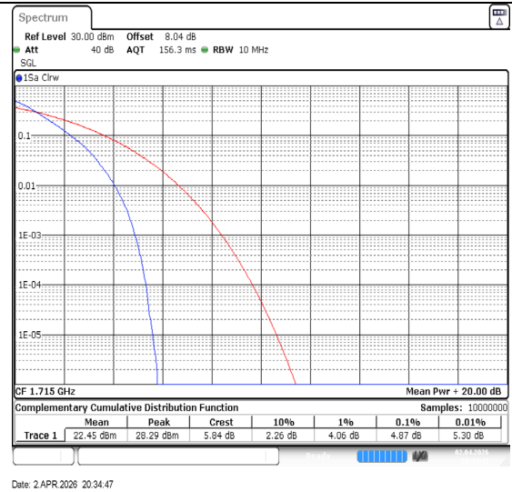
Band66-10MHz-QPSK-132022-50RB#0-PASS
