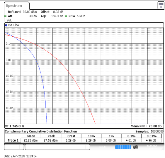
Band66-5MHz-QPSK-132322-25RB#0-PASS
