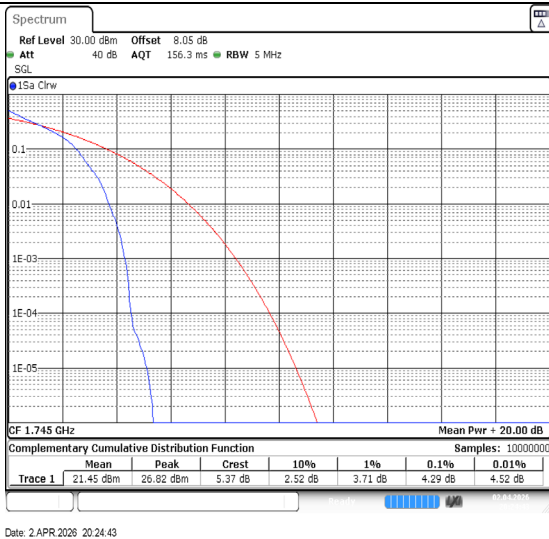
Band66-5MHz-QPSK-132322-1RB#0-PASS
