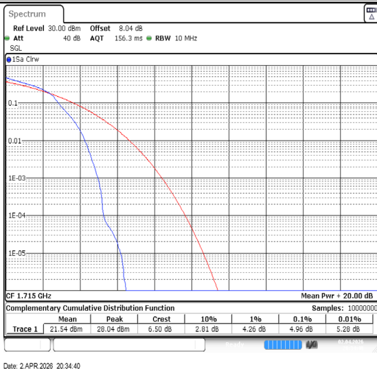
Band66-10MHz-16QAM-132022-1RB#0-PASS
