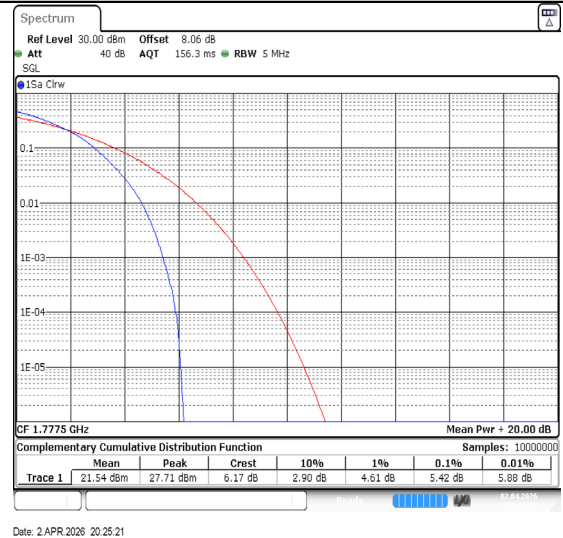
Band66-5MHz-16QAM-132647-25RB#0-PASS
