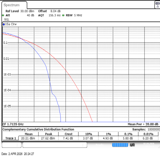
Band66-5MHz-64QAM-131997-1RB#0-PASS
