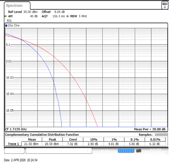
Band66-5MHz-16QAM-131997-25RB#0-PASS
