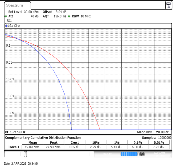
Band66-10MHz-64QAM-132022-50RB#0-PASS
