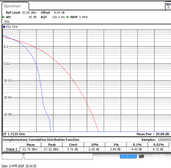
Band66-5MHz-QPSK-131997-1RB#0-PASS
