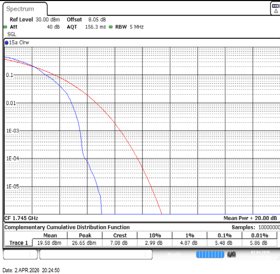
Band66-5MHz-64QAM-132322-1RB#0-PASS
