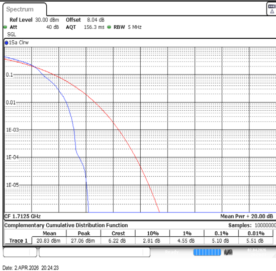
Band66-5MHz-16QAM-131997-1RB#0-PASS
