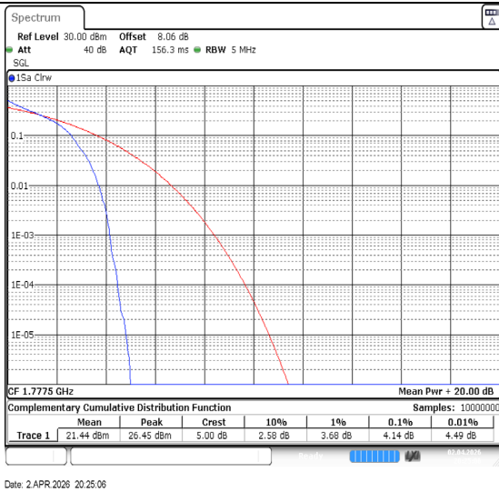
Band66-5MHz-QPSK-132647-1RB#0-PASS
