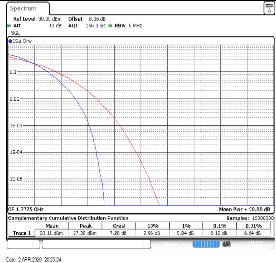
Band66-5MHz-64QAM-132647-25RB#0-PASS
