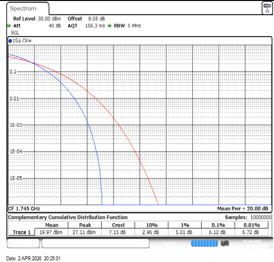
Band66-5MHz-64QAM-132322-25RB#0-PASS
