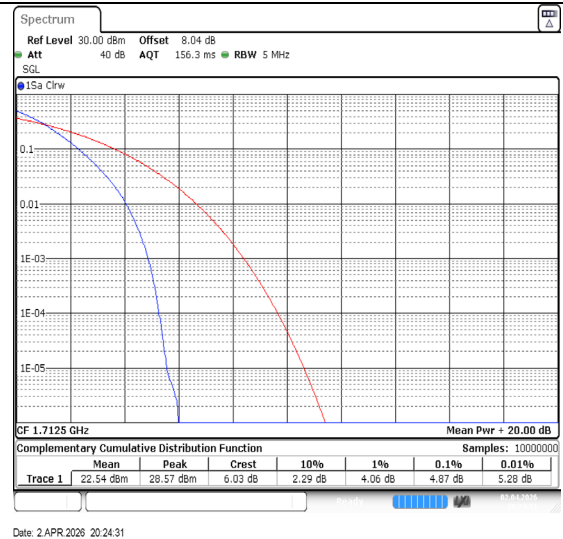
Band66-5MHz-QPSK-131997-25RB#0-PASS
