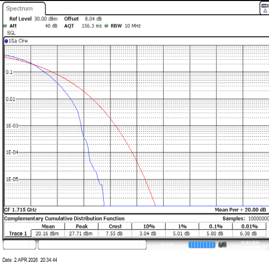
Band66-10MHz-64QAM-132022-1RB#0-PASS
