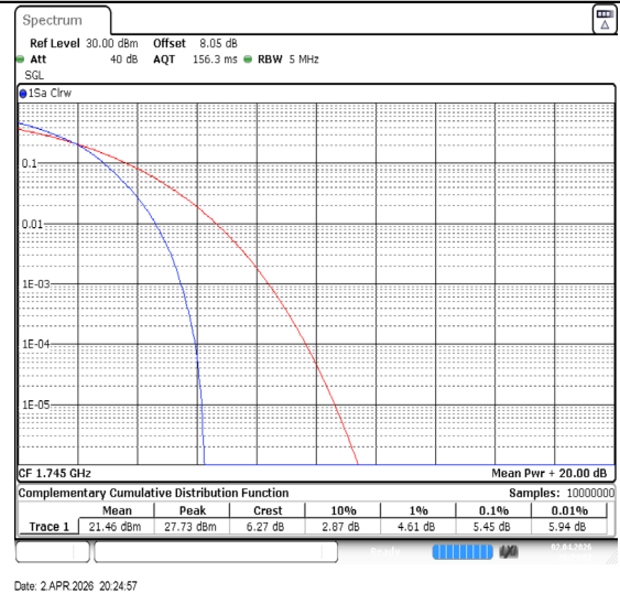
Band66-5MHz-16QAM-132322-25RB#0-PASS
