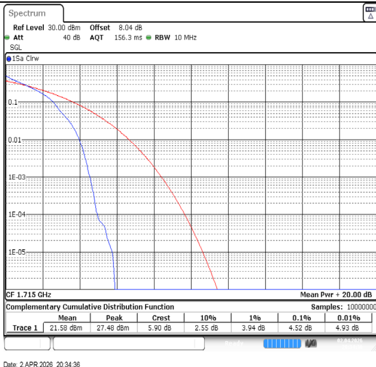
Band66-10MHz-QPSK-132022-1RB#0-PASS
