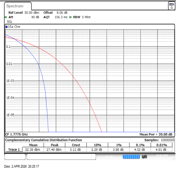
Band66-5MHz-QPSK-132647-25RB#0-PASS
