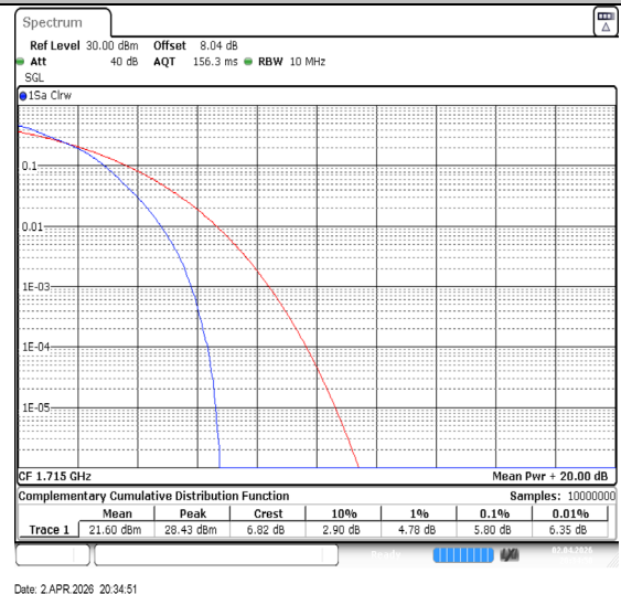
Band66-10MHz-16QAM-132022-50RB#0-PASS
