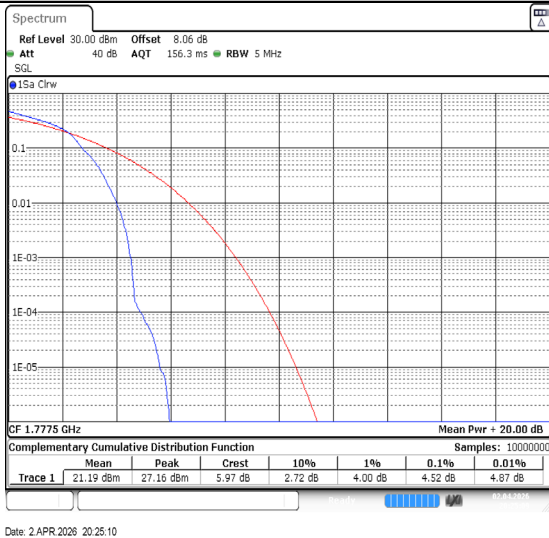
Band66-5MHz-16QAM-132647-1RB#0-PASS
