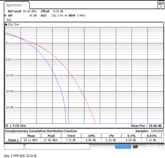
Band66-5MHz-64QAM-131997-25RB#0-PASS
