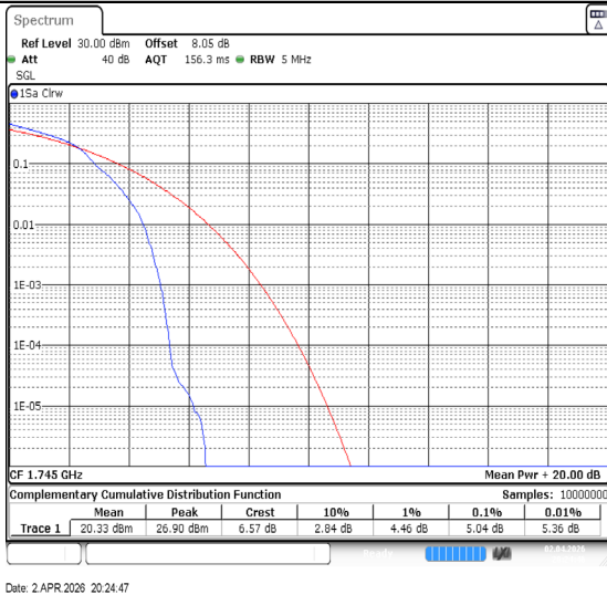
Band66-5MHz-16QAM-132322-1RB#0-PASS
