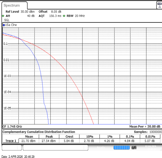
Band66-15MHz-16QAM-132322-1RB#0-PASS
