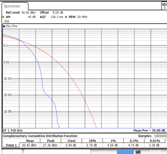
Band66-20MHz-64QAM-132322-1RB#0-PASS
