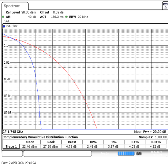
Band66-15MHz-QPSK-132322-1RB#0-PASS
