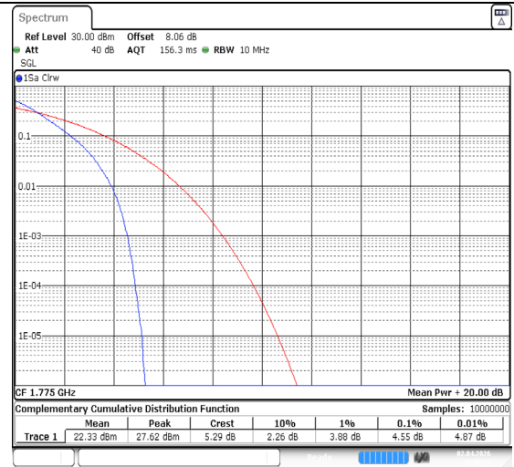
Band66-10MHz-QPSK-132622-50RB#0-PASS
