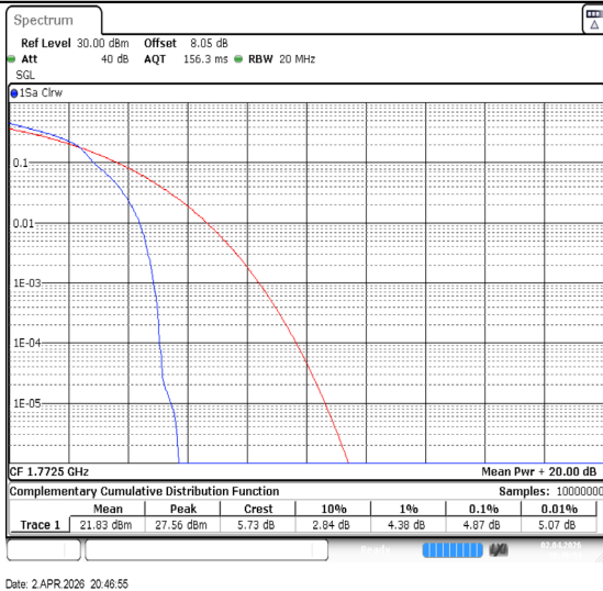
Band66-15MHz-16QAM-132597-1RB#0-PASS
