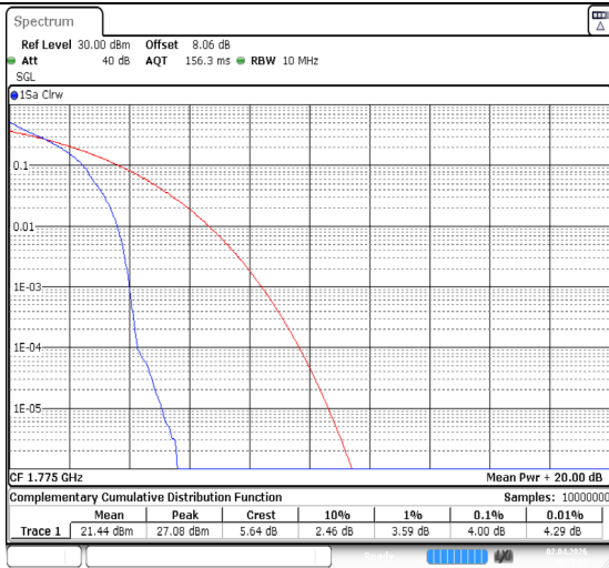
Band66-10MHz-QPSK-132622-1RB#0-PASS
