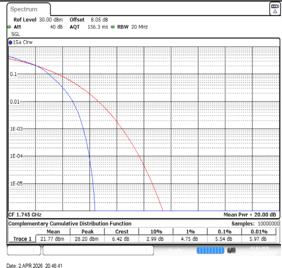
Band66-15MHz-16QAM-132322-75RB#0-PASS
