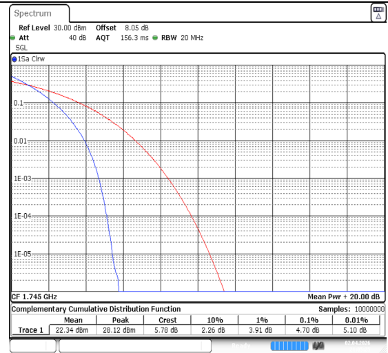
Band66-20MHz-QPSK-132322-100RB#0-PASS
