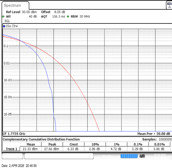
Band66-15MHz-64QAM-132597-1RB#0-PASS
