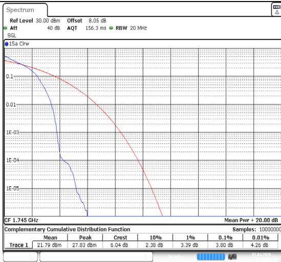
Band66-20MHz-QPSK-132322-1RB#0-PASS
