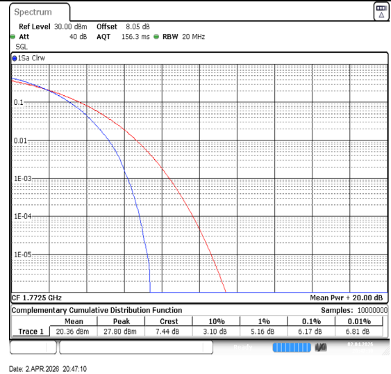
Band66-15MHz-64QAM-132597-75RB#0-PASS
