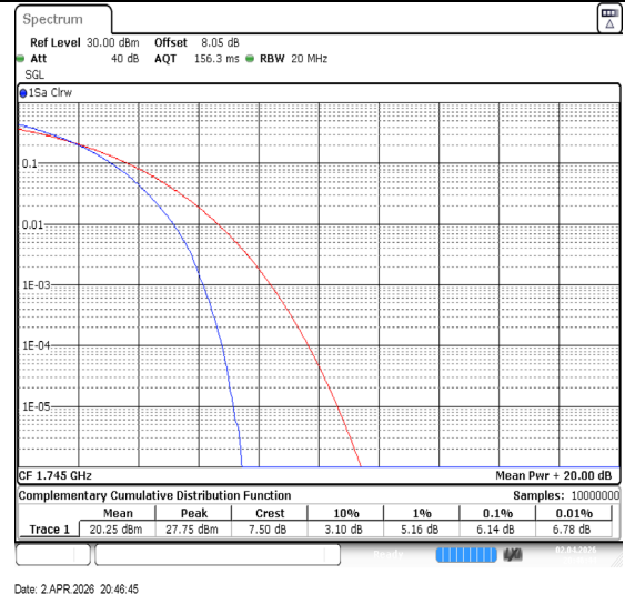
Band66-15MHz-64QAM-132322-75RB#0-PASS
