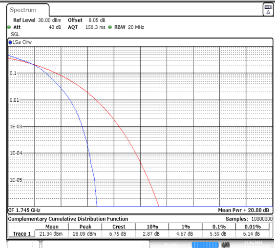
Band66-20MHz-64QAM-132322-100RB#0-PASS
