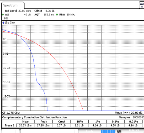
Band66-10MHz-64QAM-132622-1RB#0-PASS
