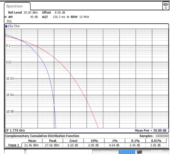
Band66-10MHz-64QAM-132622-50RB#0-PASS
