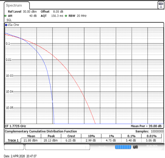
Band66-15MHz-16QAM-132597-75RB#0-PASS
