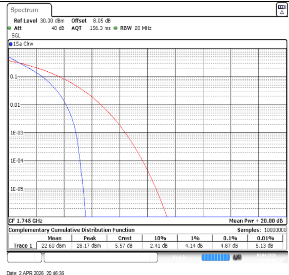
Band66-15MHz-QPSK-132322-75RB#0-PASS
