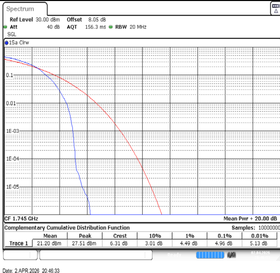
Band66-15MHz-64QAM-132322-1RB#0-PASS
