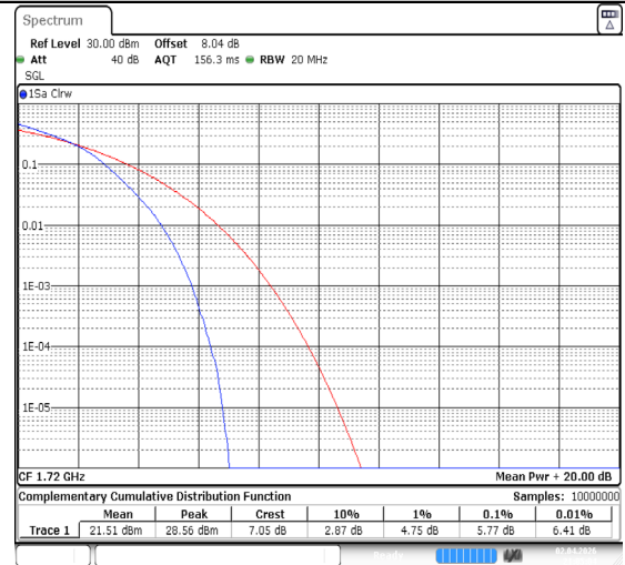
Band66-20MHz-QPSK-132072-100RB#0-PASS
