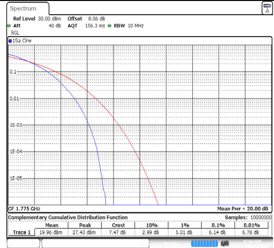
Band66-10MHz-QPSK-132622-50RB#0-PASS
