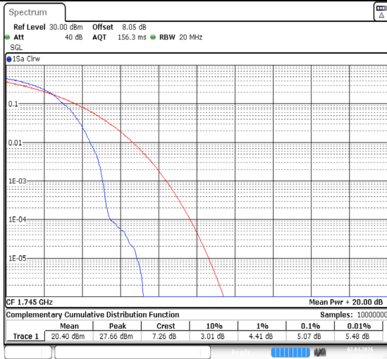
Band66-20MHz-QPSK-132322-1RB#0-PASS
