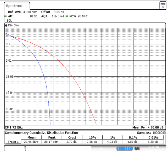
Band66-20MHz-QPSK-132072-100RB#0-PASS
