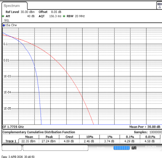
Band66-15MHz-QPSK-132597-1RB#0-PASS
