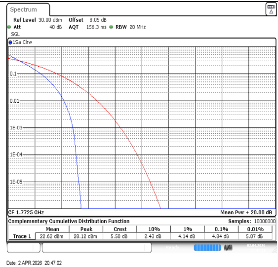
Band66-15MHz-QPSK-132597-75RB#0-PASS
