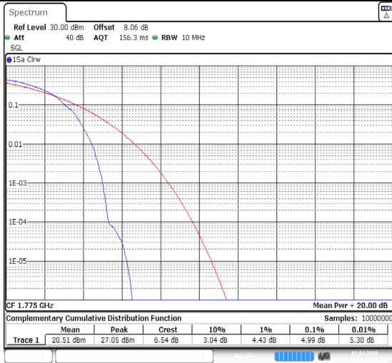
Band66-10MHz-QPSK-132622-1RB#0-PASS
