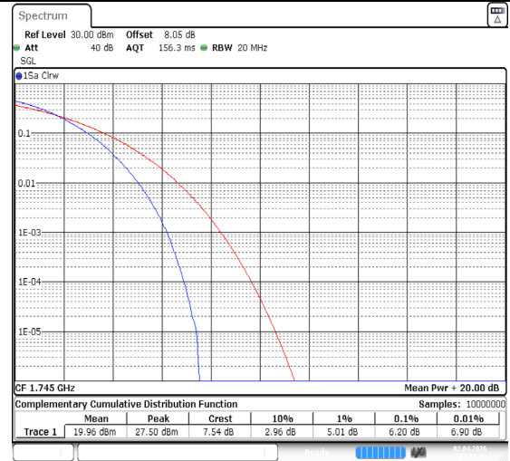
Band66-20MHz-QPSK-132322-100RB#0-PASS
