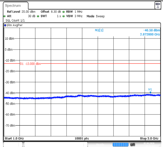
Band13-5MHz-QPSK-23205-25RB#0-1000~3000-PASS
