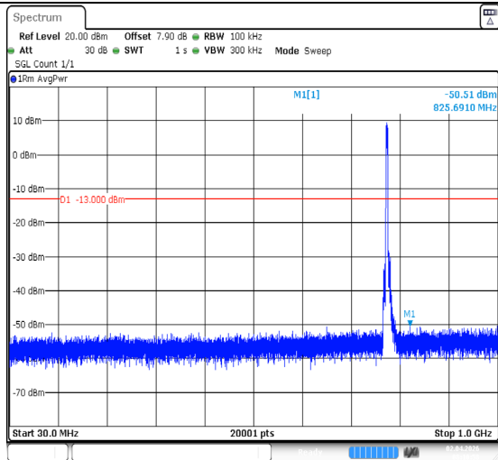
Band13-5MHz-QPSK-23205-25RB#0-30~1000-PASS
