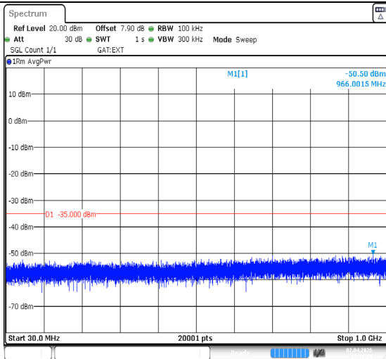
Band38-5MHz-QPSK-38225-1RB#0-30~1000-PASS
