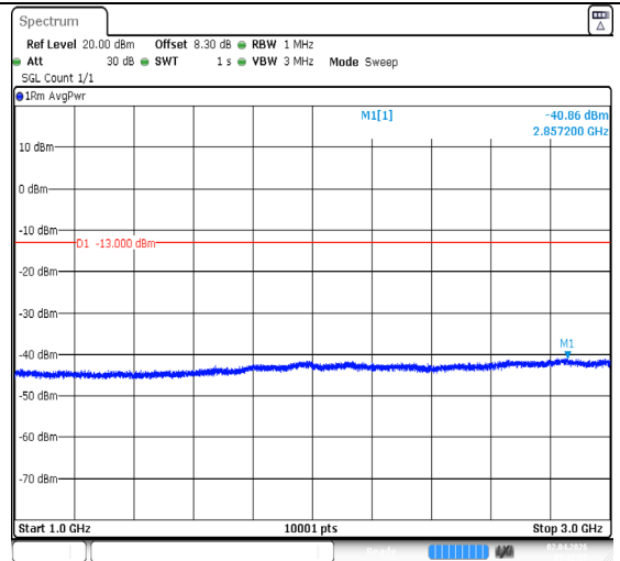
Band13-5MHz-QPSK-23255-1RB#0-1000~3000-PASS
