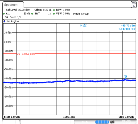
Band13-5MHz-QPSK-23255-25RB#0-1000~3000-PASS
