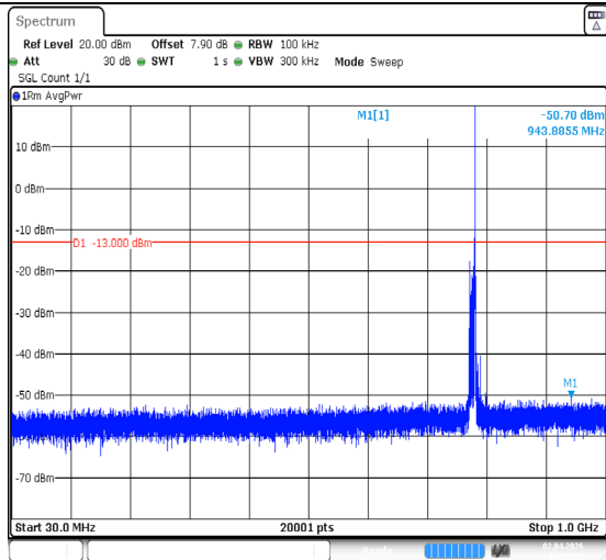
Band13-10MHz-QPSK-23230-1RB#49-30~1000-PASS
