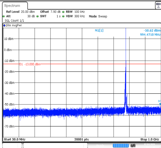
Band13-5MHz-QPSK-23230-1RB#24-30~1000-PASS
