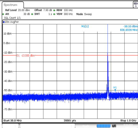
Band13-5MHz-QPSK-23255-1RB#0-30~1000-PASS
