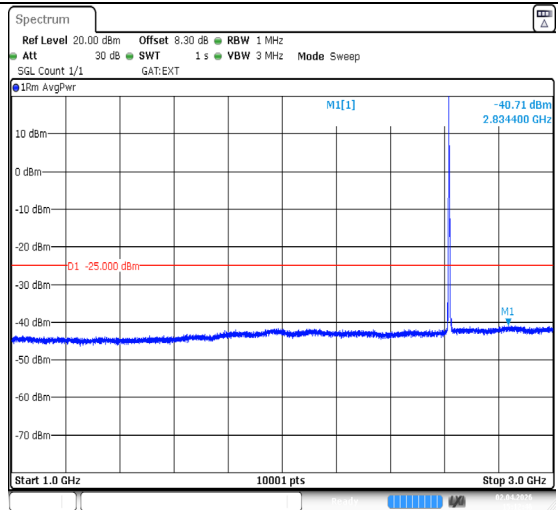
Band38-5MHz-QPSK-38225-1RB#0-1000~3000-PASS
