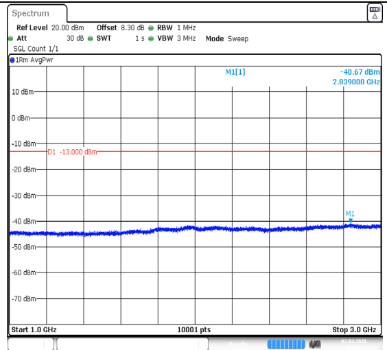
Band13-5MHz-QPSK-23230-1RB#24-1000~3000-PASS
