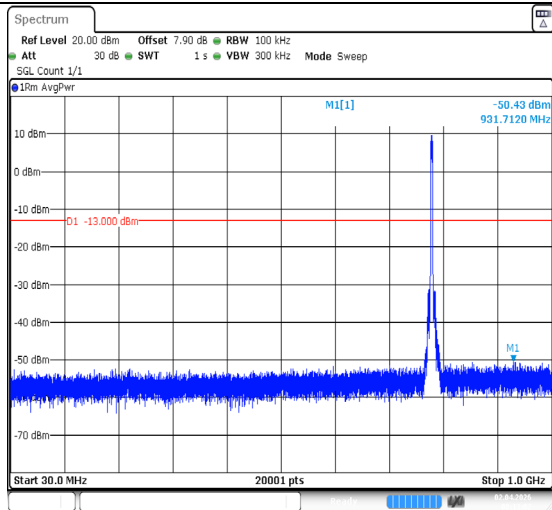
Band13-5MHz-QPSK-23255-25RB#0-30~1000-PASS
