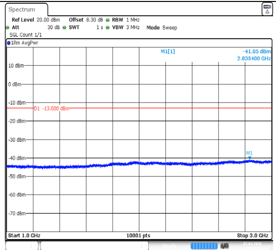
Band13-10MHz-QPSK-23230-1RB#49-1000~3000-PASS
