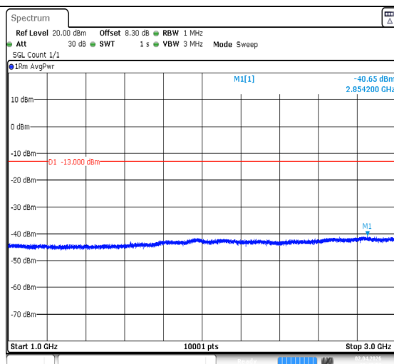
Band26(814-824)-1.4MHz-QPSK-26697-6RB#0-1000~3000-PASS
