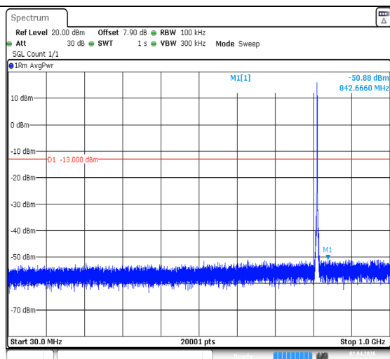
Band26(814-824)-1.4MHz-QPSK-26697-6RB#0-30~1000-PASS
