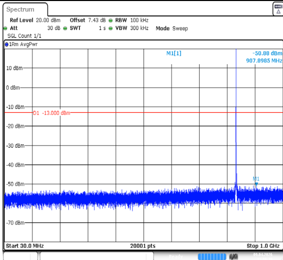
Band26(824-849)-1.4MHz-QPSK-26915-1RB#5-30~1000-PAS S
