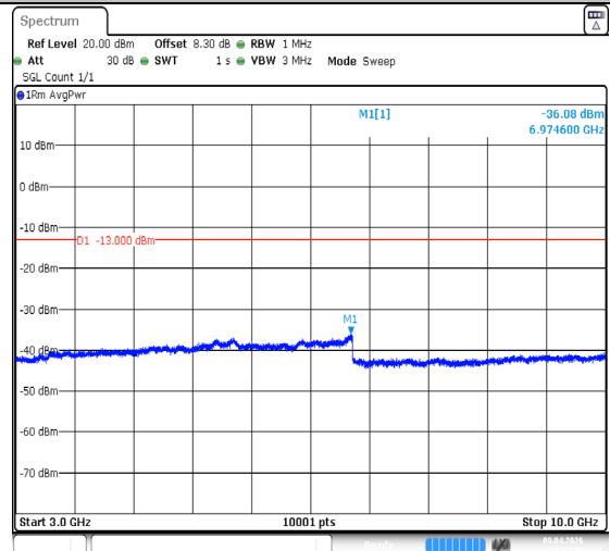
Band26(824-849)-1.4MHz-QPSK-27033-1RB#5-30~10 00-PASS
