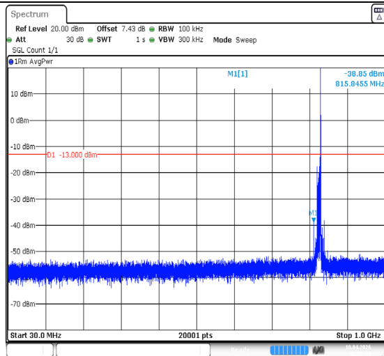
Band5-10MHz-QPSK-20450-1RB#49-30~1000-PASS
