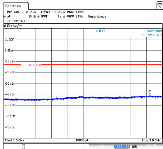
Band5-10MHz-QPSK-20450-1RB#49-1000~3000-PASS
