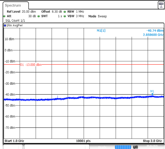
Band26(824-849)-1.4MHz-QPSK-26915-1RB#5-1000~3000-PASS
