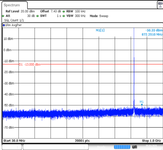
Band26(824-849)-1.4MHz-QPSK-26797-1RB#0-30~1000-PASS
