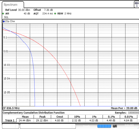
Band5-1.4MHz-QPSK-20525-1RB#0-PASS
