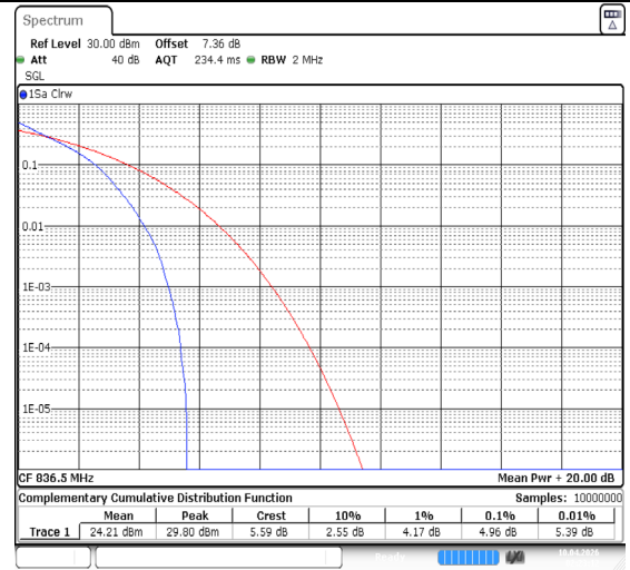
Band5-1.4MHz-QPSK-20525-6RB#0-PASS
