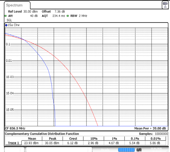
Band5-1.4MHz-64QAM-20525-6RB#0-PASS
