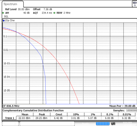
Band5-1.4MHz-QPSK-20525-1RB#0-PASS
