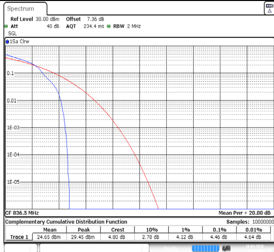
Band5-1.4MHz-64QAM-20525-1RB#0-PASS
