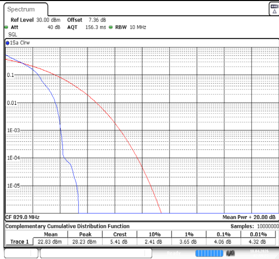
Band5-10MHz-QPSK-20450-1RB#0-PASS
