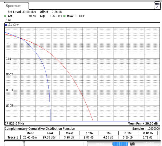
Band5-10MHz-64QAM-20450-50RB#0-PASS
