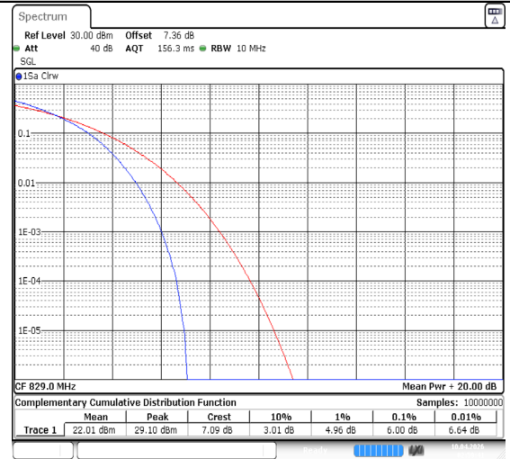
Band5-10MHz-QPSK-20450-50RB#0-PASS
