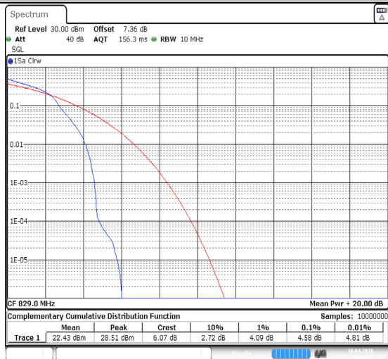
Band5-10MHz-64QAM-20450-1RB#0-PASS
