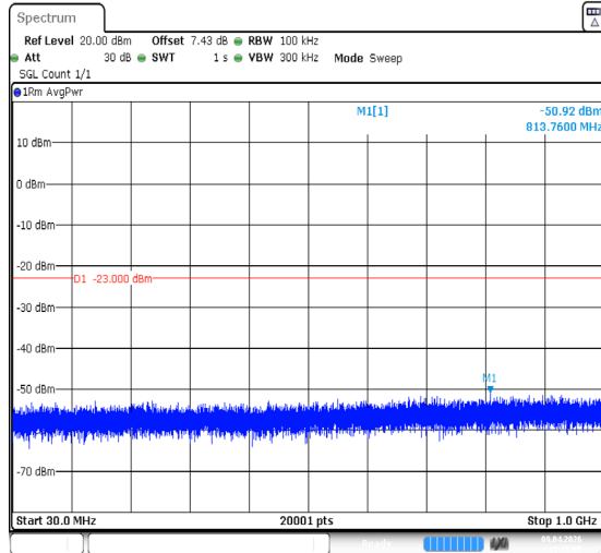
Band2-20MHz-QPSK-18900-100RB#0-30~1000-PASS
