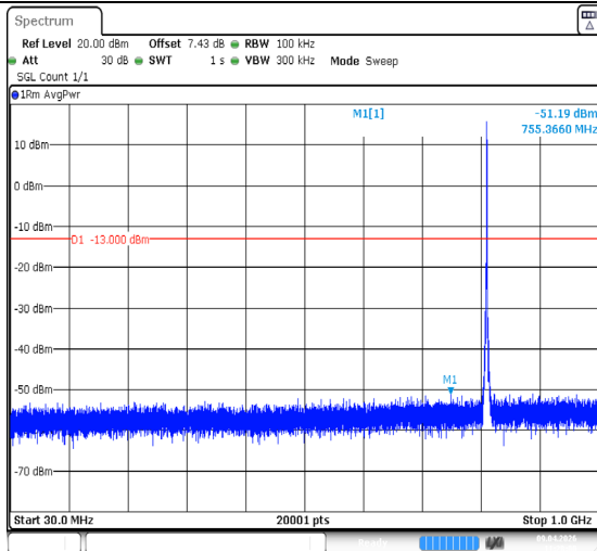
Band26(814-824)-1.4MHz-QPSK-26697-6RB#0-30~1000-PASS
