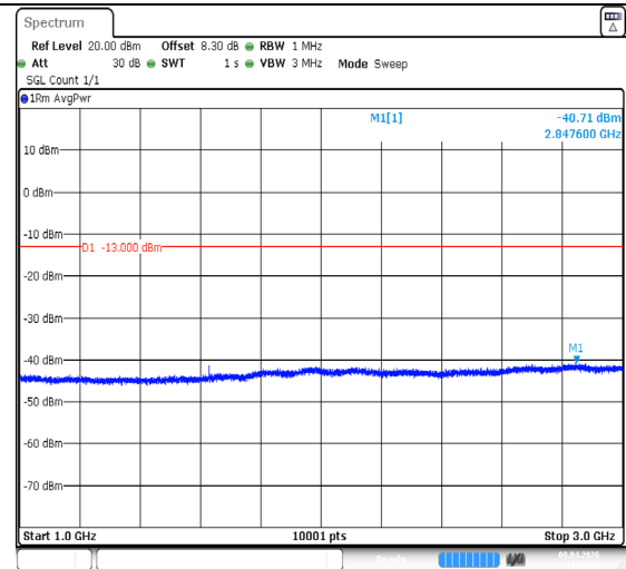
Band26(814-824)-1.4MHz-QPSK-26697-1RB#0-1000~3000-PASS
