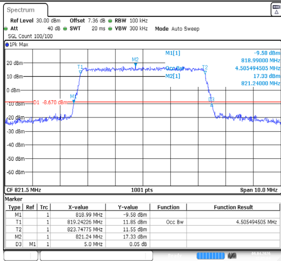
Band26(814-824)-5MHz-QPSK-26765-25RB#0-PASS
