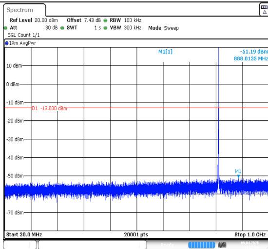
Band26(814-824)-1.4MHz-QPSK-26697-1RB#0-30~1000-PASS
