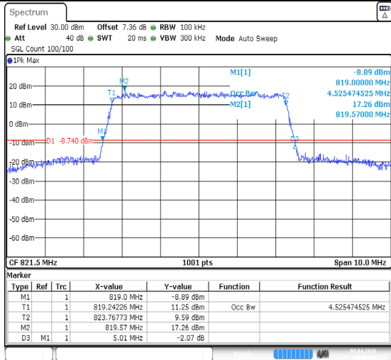
Band26(814-824)-5MHz-QPSK-26765-25RB#0-PASS
