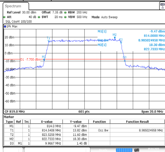
Band26(814-824)-10MHz-QPSK-26740-50RB#0-PASS
