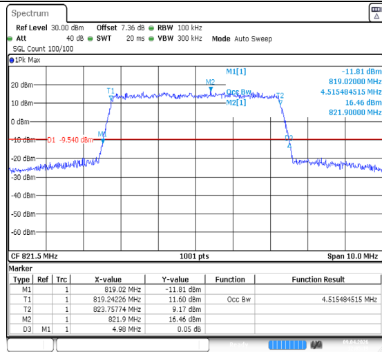
Band26(814-824)-5MHz-64QAM-26765-25RB#0-PASS
