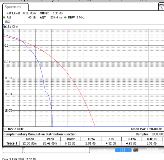
Band26(814-824)-3MHz-16QAM-26775-1RB#0-PASS
