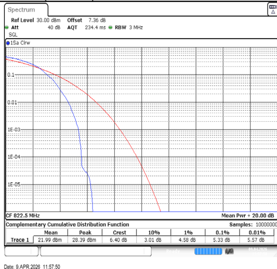
Band26(814-824)-3MHz-64QAM-26775-1RB#0-PASS
