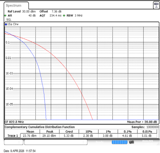
Band26(814-824)-3MHz-QPSK-26775-15RB#0-PASS
