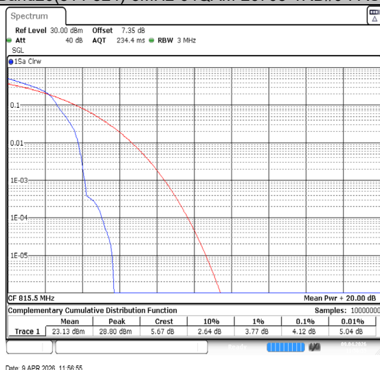
Band26(814-824)-3MHz-16QAM-26705-1RB#0-PASS
