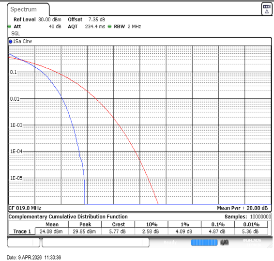
Band26(814-824)-1.4MHz-QPSK-26740-6RB#0-PASS
