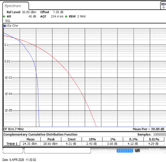
Band26(814-824)-1.4MHz-QPSK-26697-1RB#0-PASS
