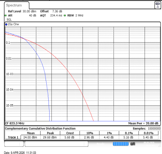
Band26(814-824)-1.4MHz-16QAM-26783-6RB#0-PASS
