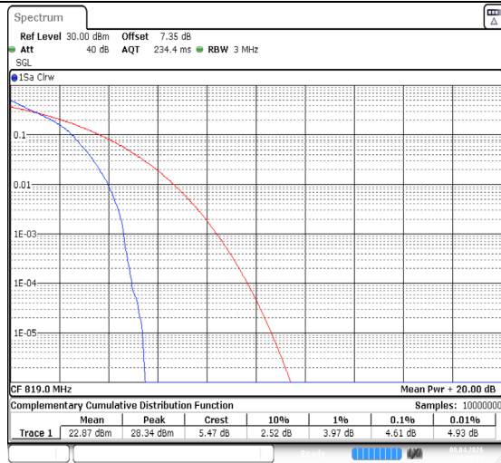
Band26(814-824)-3MHz-QPSK-26740-1RB#0-PASS
