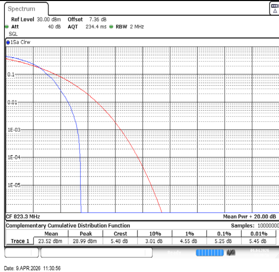
Band26(814-824)-1.4MHz-64QAM-26783-1RB#0-PASS
