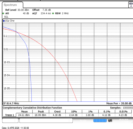
Band26(814-824)-1.4MHz-16QAM-26697-1RB#0-PASS
