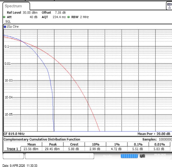
Band26(814-824)-1.4MHz-64QAM-26740-1RB#0-PASS
