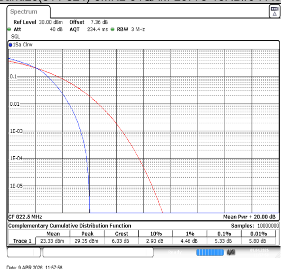
Band26(814-824)-3MHz-16QAM-26775-15RB#0-PASS
