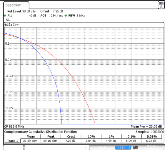
Band26(814-824)-3MHz-QPSK-26740-15RB#0-PASS
