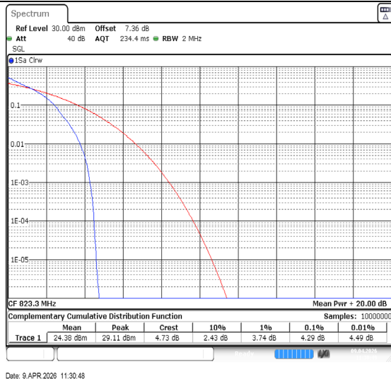
Band26(814-824)-1.4MHz-QPSK-26783-1RB#0-PASS
