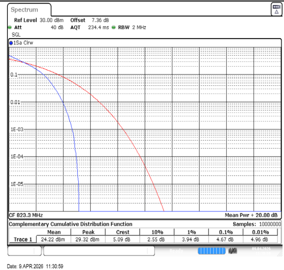
Band26(814-824)-1.4MHz-QPSK-26783-6RB#0-PASS
