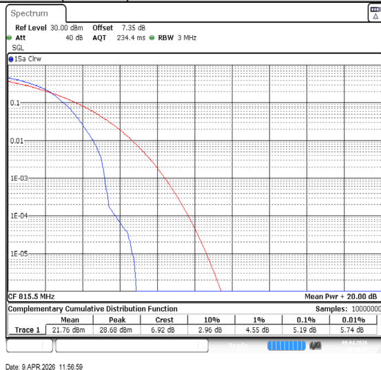
Band26(814-824)-3MHz-64QAM-26705-1RB#0-PASS
