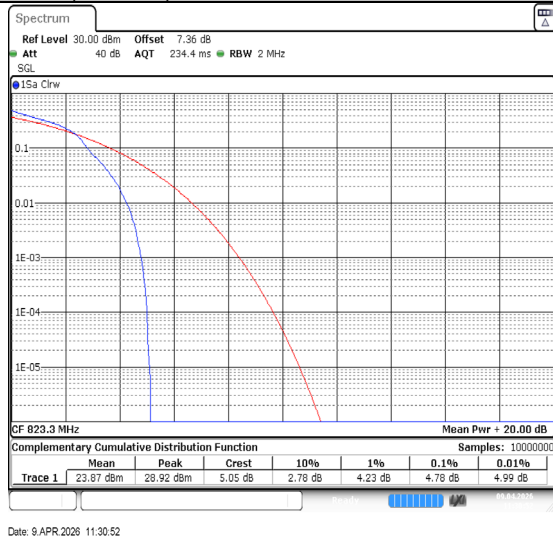
Band26(814-824)-1.4MHz-16QAM-26783-1RB#0-PASS
