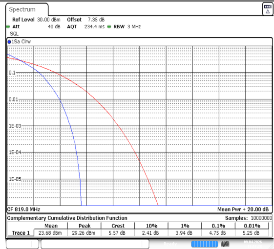
Band26(814-824)-3MHz-QPSK-26740-15RB#0-PASS
