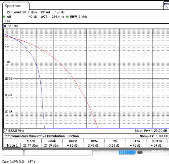
Band26(814-824)-3MHz-QPSK-26775-1RB#0-PASS
