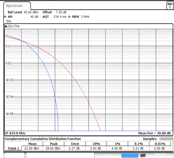
Band26(814-824)-3MHz-64QAM-26740-15RB#0-PASS
