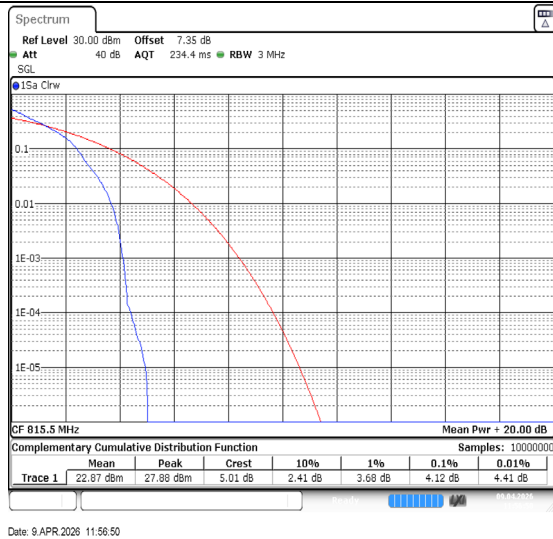
Band26(814-824)-3MHz-QPSK-26705-1RB#0-PASS
