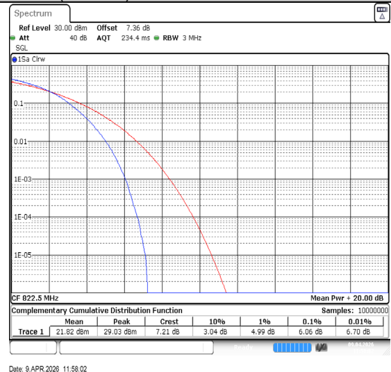
Band26(814-824)-3MHz-64QAM-26775-15RB#0-PASS
