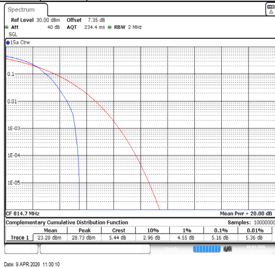
Band26(814-824)-1.4MHz-64QAM-26697-1RB#0-PASS
