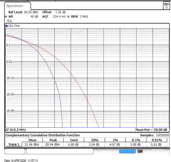
Band26(814-824)-3MHz-64QAM-26705-15RB#0-PASS
