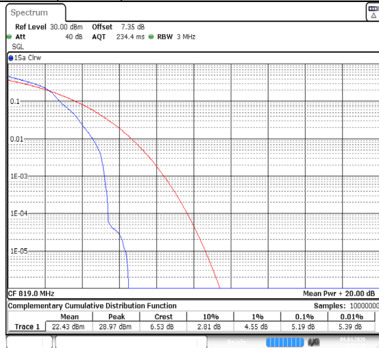
Band26(814-824)-3MHz-64QAM-26740-1RB#0-PASS
