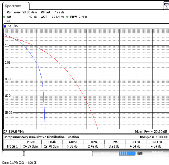
Band26(814-824)-1.4MHz-QPSK-26740-1RB#0-PASS
