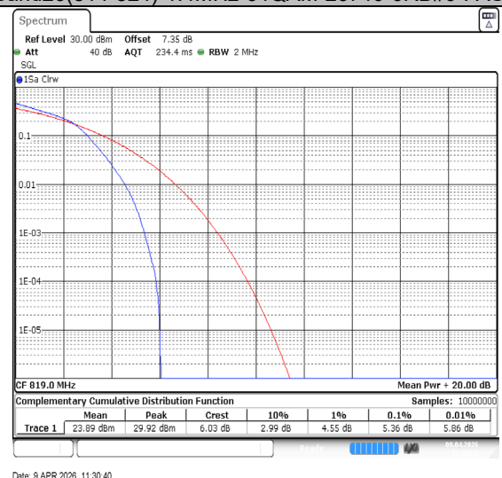
Band26(814-824)-1.4MHz-16QAM-26740-6RB#0-PASS
