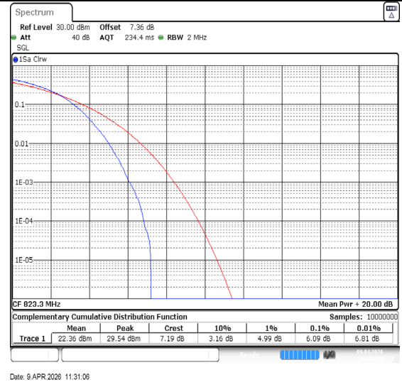
Band26(814-824)-1.4MHz-64QAM-26783-6RB#0-PASS
