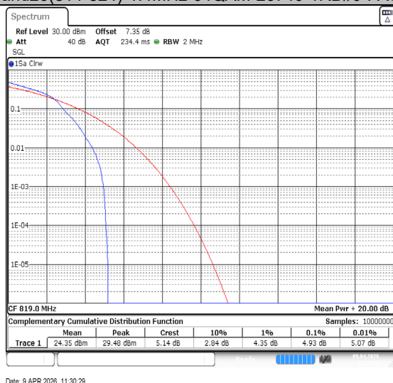
Band26(814-824)-1.4MHz-16QAM-26740-1RB#0-PASS
