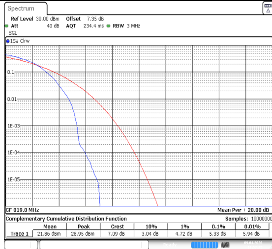
Band26(814-824)-3MHz-QPSK-26740-1RB#0-PASS
