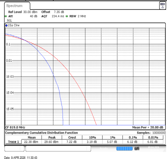
Band26(814-824)-1.4MHz-64QAM-26740-6RB#0-PASS
