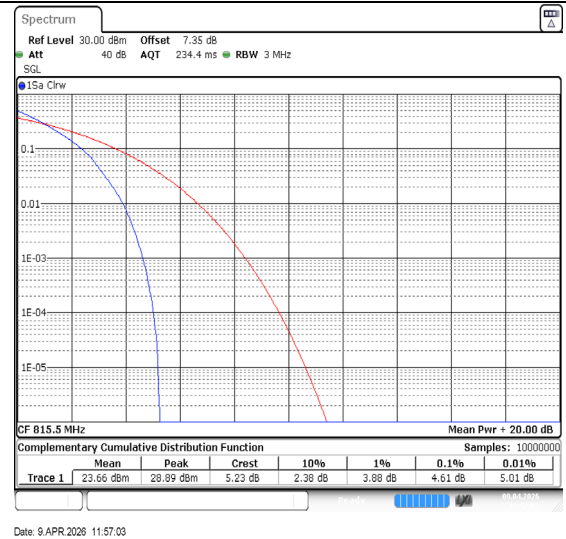
Band26(814-824)-3MHz-QPSK-26705-15RB#0-PASS
