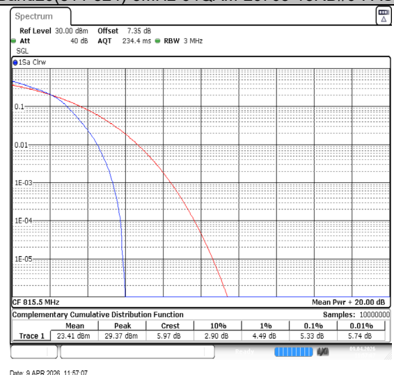
Band26(814-824)-3MHz-16QAM-26705-15RB#0-PASS
