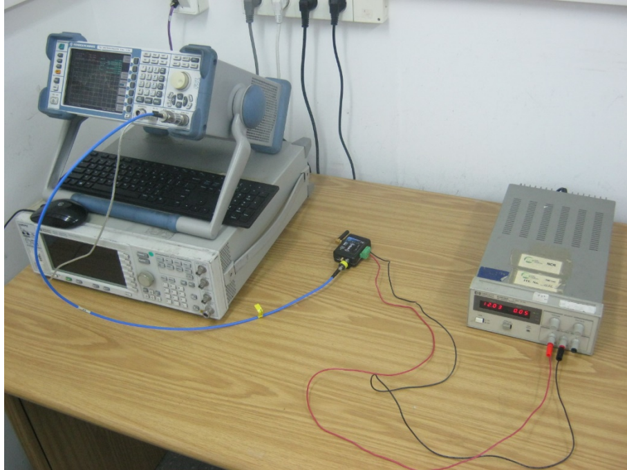
Conducted Emission from Antenna Port
