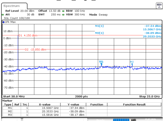
BLE_2M_High_Channel
