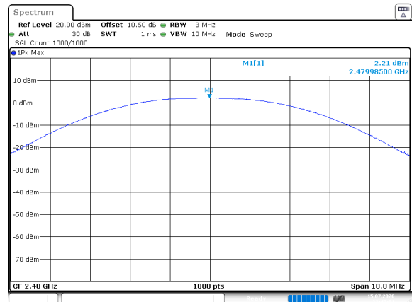
BLE_2M_High_Channel
