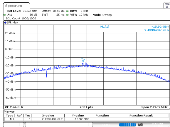
BLE_2M_Middle_Channel
