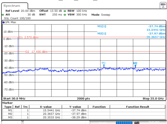
BLE_2M_Low_Channel
