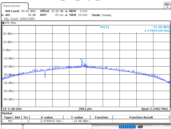
BLE_2M_High_Channel
