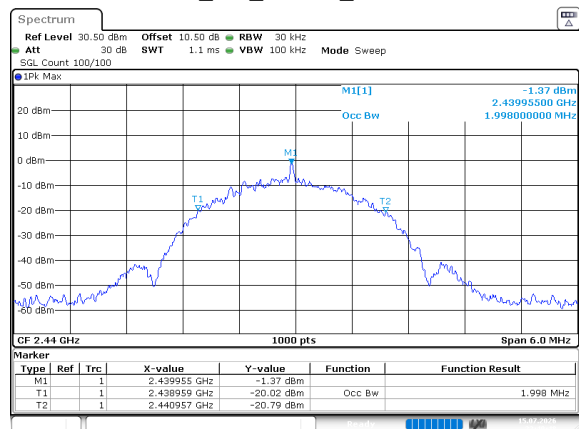
BLE_2M_Middle_Channel
