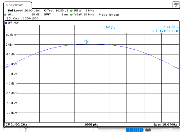
BLE_2M_Low_Channel
