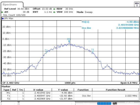
BLE_2M_Low_Channel
