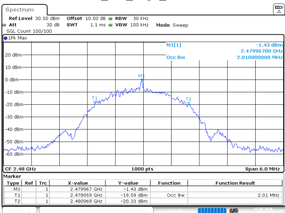
BLE_2M_High_Channel
