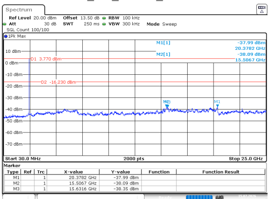
BLE_2M_Middle_Channel
