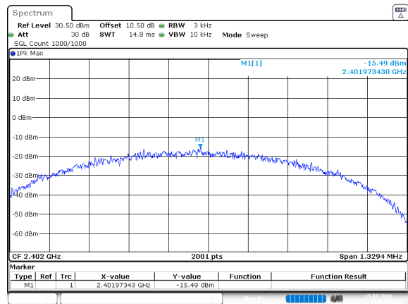
BLE_1M_Low_Channel
