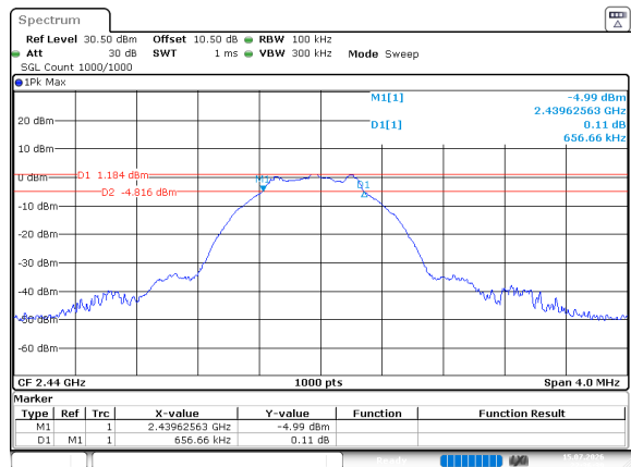
BLE_1M_Middle_Channel
