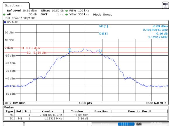
BLE_2M_Low_Channel
