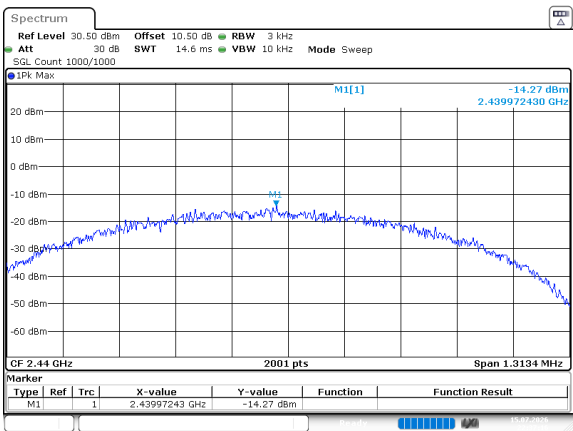
BLE_1M_Middle_Channel
