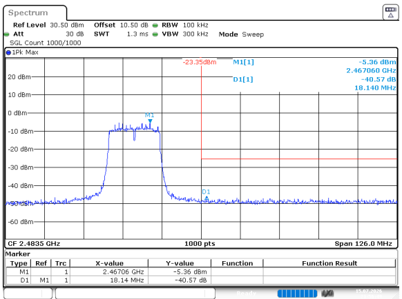
802.11g_2462MHz
