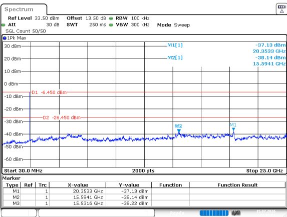
802.11g_2412MHz
