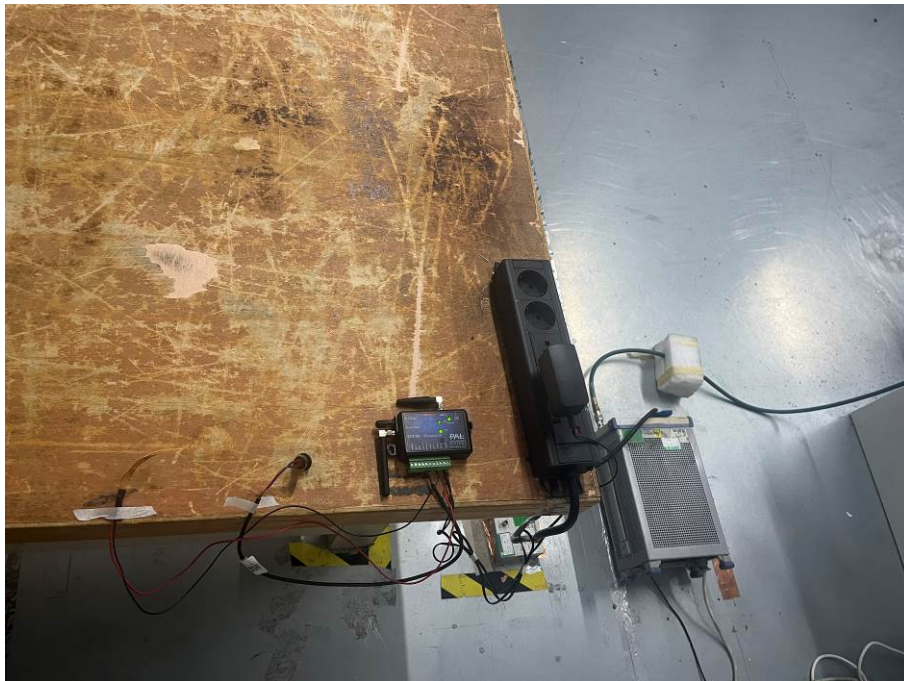
Conducted Emissions - Side View_SPIDER - Wiegand 26
