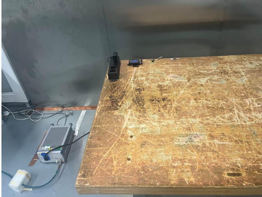
Conducted Emissions - Front View_SPIDER - Wiegand 26
