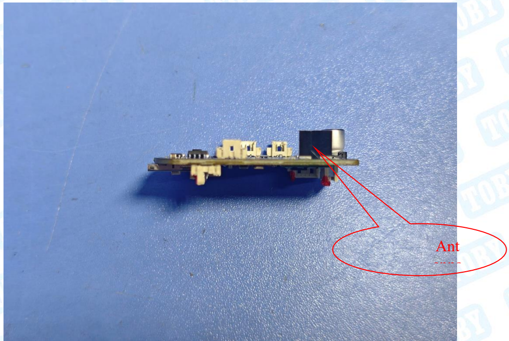
Photo 18 Internal of EUT--without shielding covers
