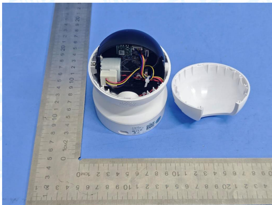
Photo 18 Internal of EUT--without shielding covers
