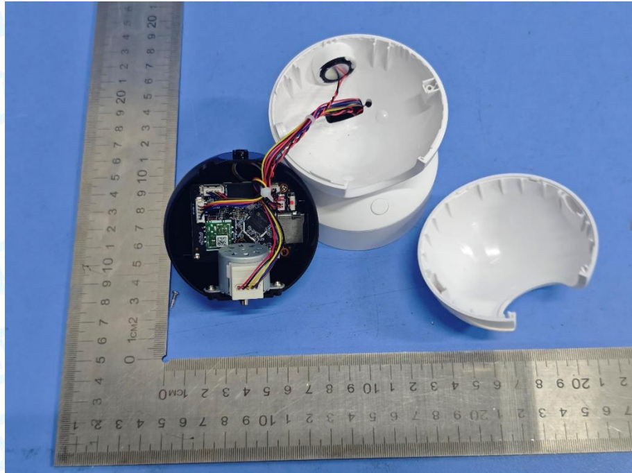
Photo 20 Internal of EUT--without shielding covers
