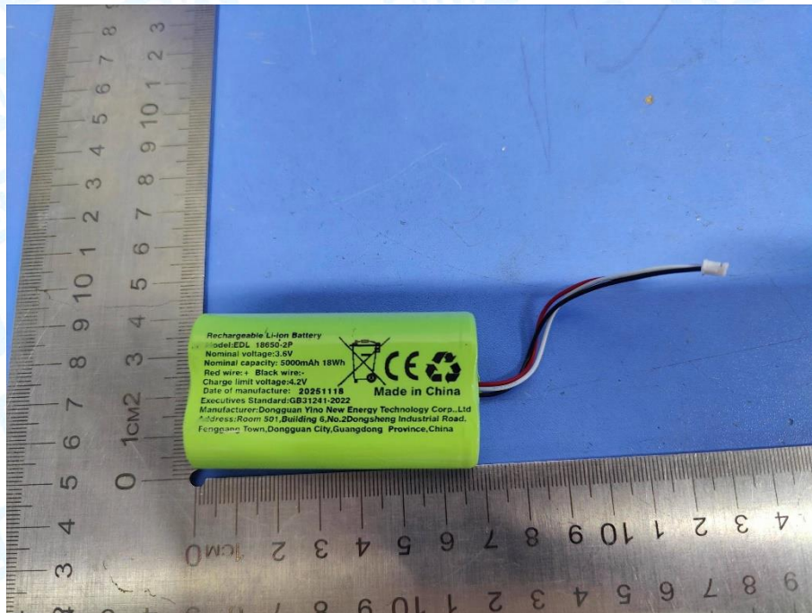
Photo 13 Battery Appearance
