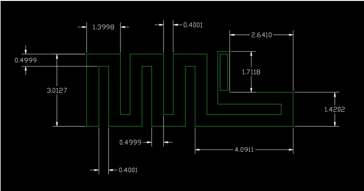
Picture of antenna
